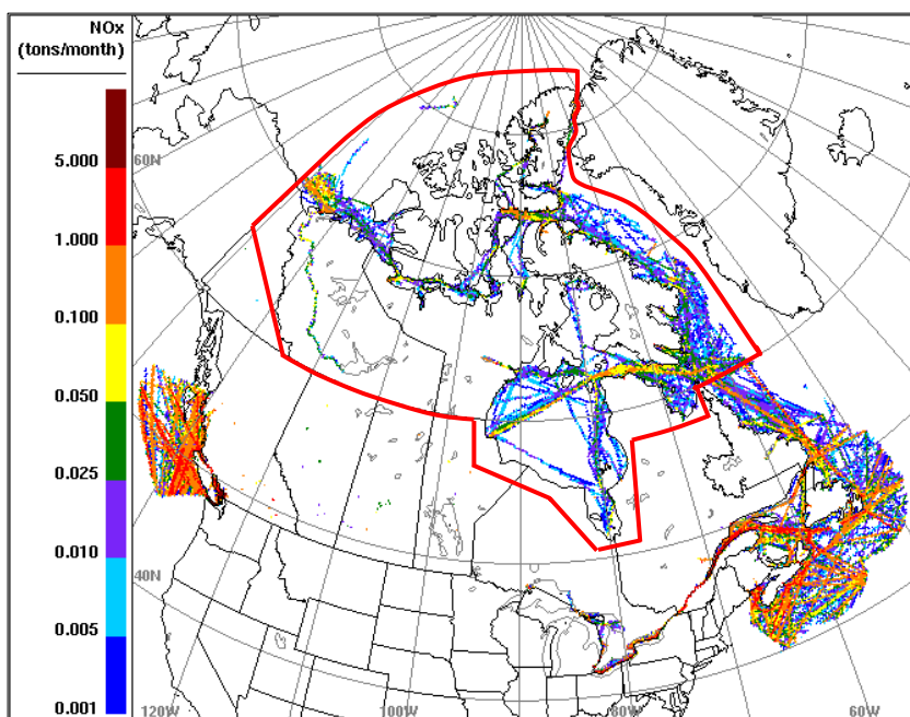
10 Figure 2. Processed model-ready \text{NO}_x marine shipping emissions for August 2010 zoomed over Canadian waters, the red line outlining the Arctic region (including Hudson Bay) which is excluded from the current North American ECA designation.
