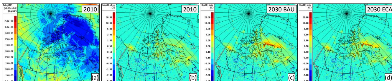
Figure 19. Modelled total BC deposition flux (scaled up by 10^4 , in \text{kg m}^{-2} ) accumulated over 2010 July-August-September period (a), and relative contributions from Canadian Arctic shipping emissions: (b) 2010 base year, (c) 2030 BAU, and (d) 2030 ECA.
