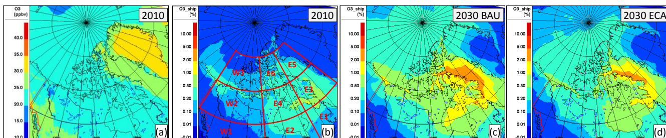
Figure 9. Modelled mean ambient O_3 concentrations for July-August-September (shipping season) for 2010 base year (a), and relative contribution from Canadian Arctic shipping emissions for the 2010 base year (b), 2030 BAU (c), and 2030 ECA (d). (The geographical subdivisions indicated on (b) are referred to in statistical assessment).
