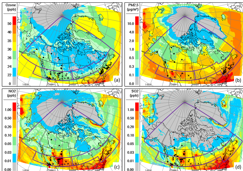
5 Figure 3. GEM-MACH Arctic modelling domain overlaid with monitoring sites: (a) O 3 monitoring sites shown on top of the modelled average ambient concentration over the July-September period; (b) same as (a) but for PM 2.5 ; (c) same as (a) but for NO 2 ; (d) same as (a) but for SO 2 . (Subdivision of regions: crosses denoting the sites in “western region”, filled triangles denoting the sites in “eastern region”, and filled circles denoting sites in the “northern region”).
