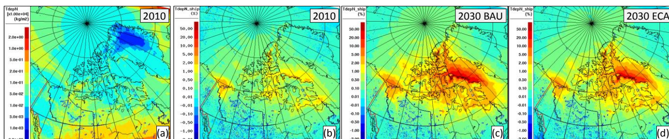
10 Figure 16. (a) Total nitrogen deposition over the July-August-September period (accumulated) for the base case (2010); (b) Arctic shipping contribution at current (2010) level; (c) as in (b) for the 2030 BAU scenario; (d) as in (b) for the 2030 ECA scenario.
