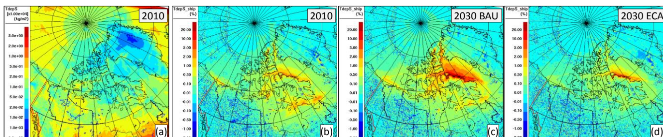
5 Figure 15. (a) Total sulphur deposition over the July-August-September period (accumulated) for the base case (2010); (b) Arctic shipping contribution at current (2010) level; (c) as in (b) for the 2030 BAU scenario; (d) as in (b) for the 2030 ECA scenario.
