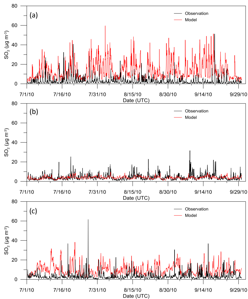
Figure 7. Regional-averaged \text{SO}_2 time series, modelled and observed: (a) northern; (b) south-western; (c) south-eastern.
