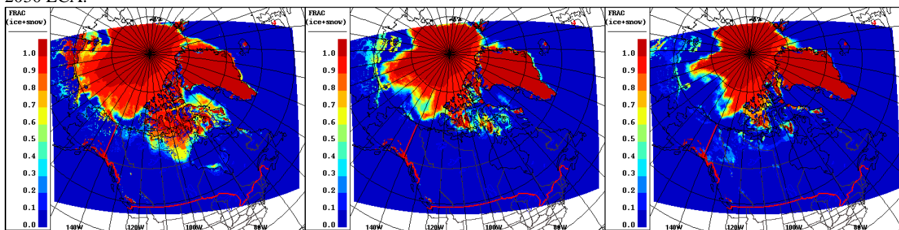
Figure 20. Monthly averaged ice/snow fraction for July, August, and September 2010.
