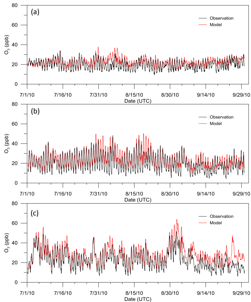
Figure 4. Regional-averaged O 3 time series, modelled and observed: (a) northern; (b) south-western; (c) south-eastern.
