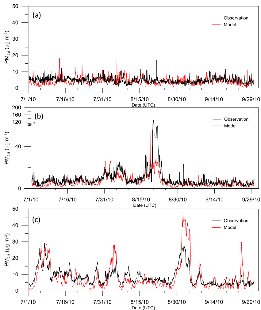
Figure 5. Regional-averaged PM 2.5 time series, modelled and observed: (a) northern; (b) south-western; (c) south-eastern.
