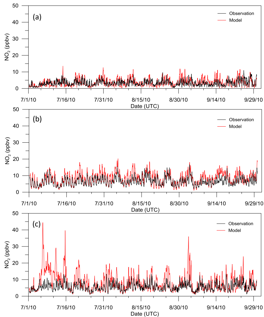
Figure 6. Regional-averaged \text{NO}_2 time series, modelled and observed: (a) northern; (b) south-western; (c) south-eastern.
