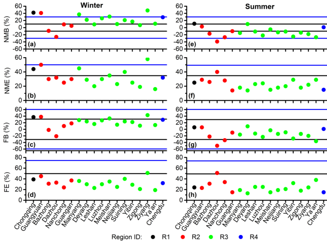
Figure S 1. Model performance for 24-hr PM_{2.5} in the 18 city centers of the SCB in the winter and summer. Note: NMB, NME, FB, and FE denote normalized mean bias, normalized mean error, fractional bias, and fractional error, respectively. The blue and black lines represent the modeling criteria and goals suggested by Emery et al. (2017), respectively. The predicted daily PM_{2.5} concentrations used to calculate NMB, NME, FB, and FE are those closest to the observations within 3x3 grid cell regions that surround the urban centers.
