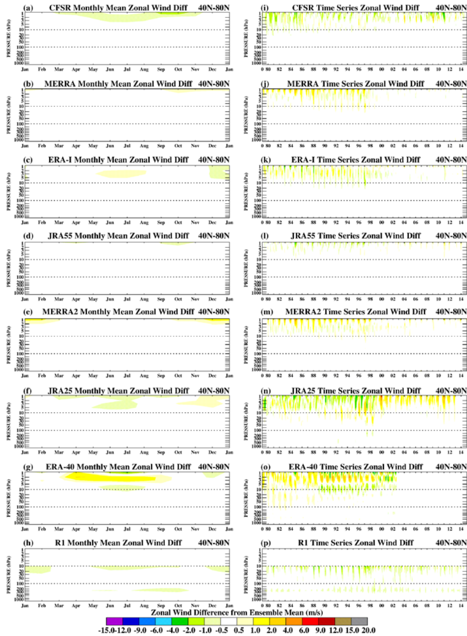
S2. Same as S1 but for the 40° N - 80° N latitude zone.
