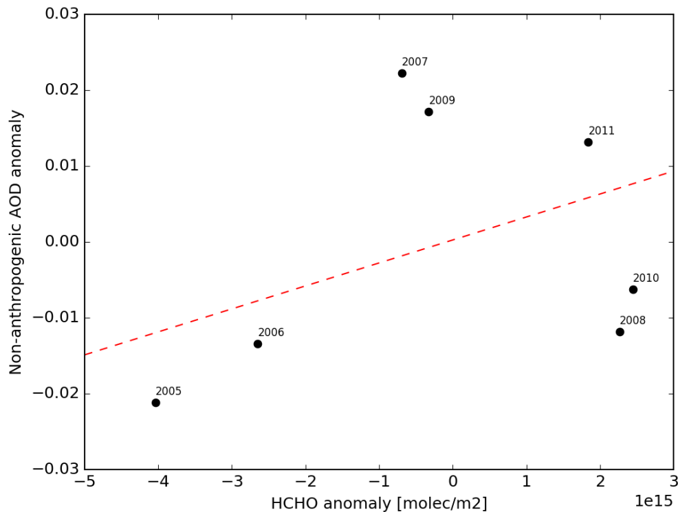
Fig. 1. Summertime anomalies in non-anthropogenic AOD vs. HCHO column, for the years 2005-2011. Non-anthropogenic AOD is based on L3 AATSR AOD and OMI tropospheric NO 2 observations. HCHO is from L2G OMI.
