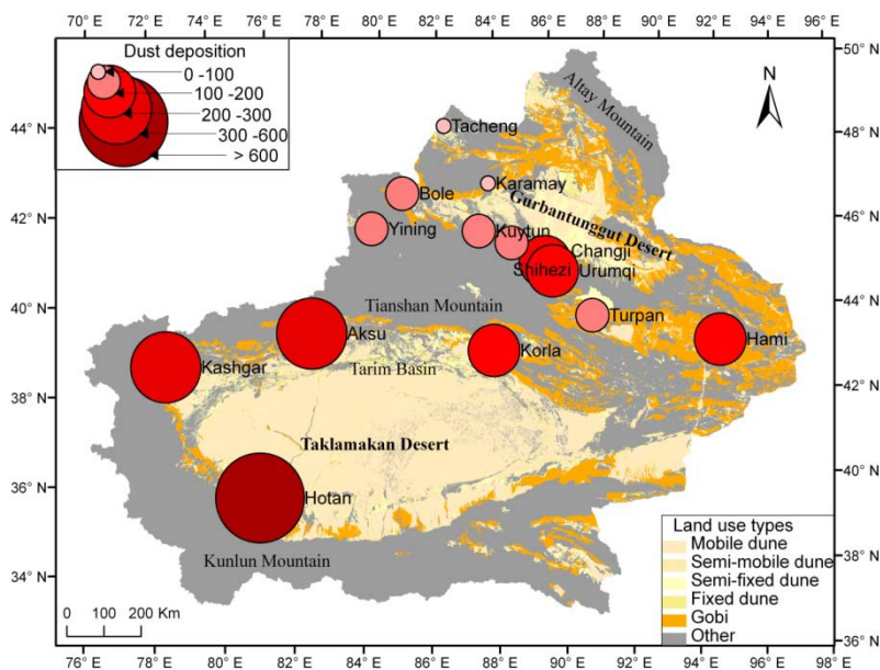
Figure 2. Annual average dust deposition ( t\ km^{-2} ) reported at 14 stations in Xinjiang Province from 2000-2013. Land use types across the province are identified according to Wang et al. (2005).
