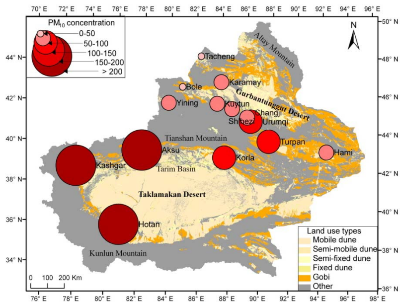
Figure 5. Annual average PM_{10} concentration ( \mu\text{g m}^{-3} ) reported for 14 stations in Xinjiang Province from 2000-2013. Land use types are identified across the province according to Wang et al., 2005.
