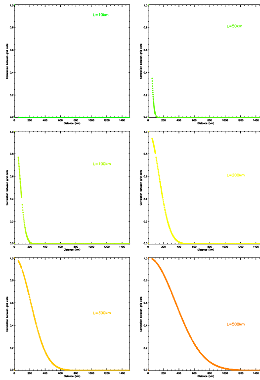
Fig. 2. Correlation between grid cells
