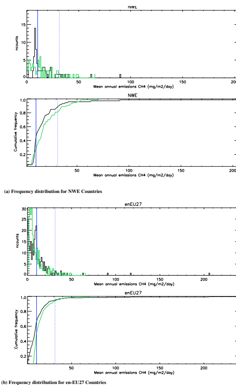
Fig. 1. Frequency distributions of prior and true emissions
