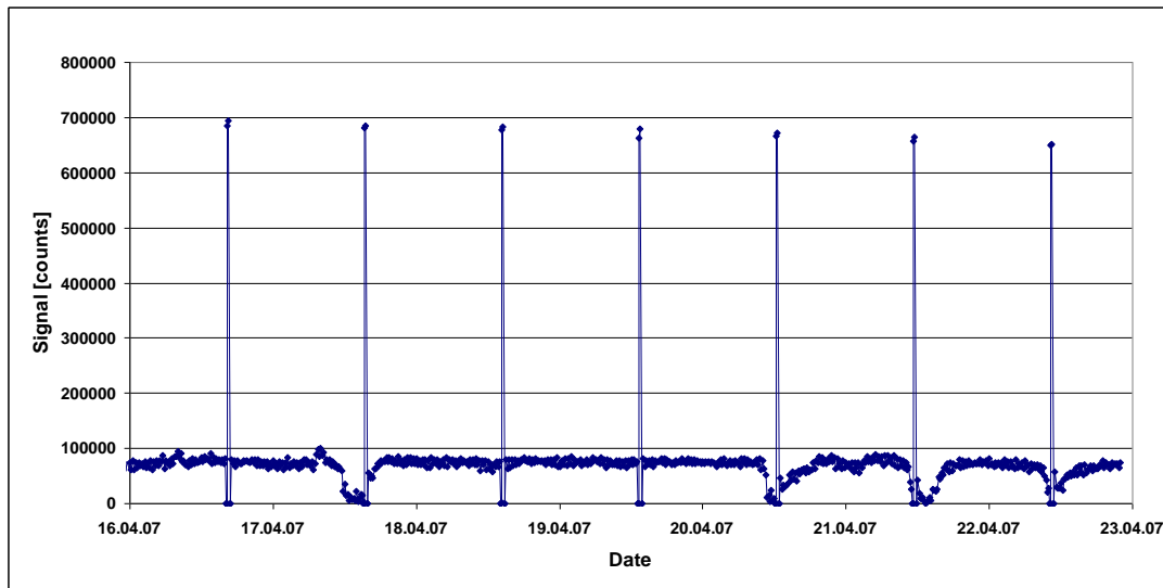
Fig. 1: Raw signal of the Tekran instrument at Cape Point in April 16–22, 2007.
