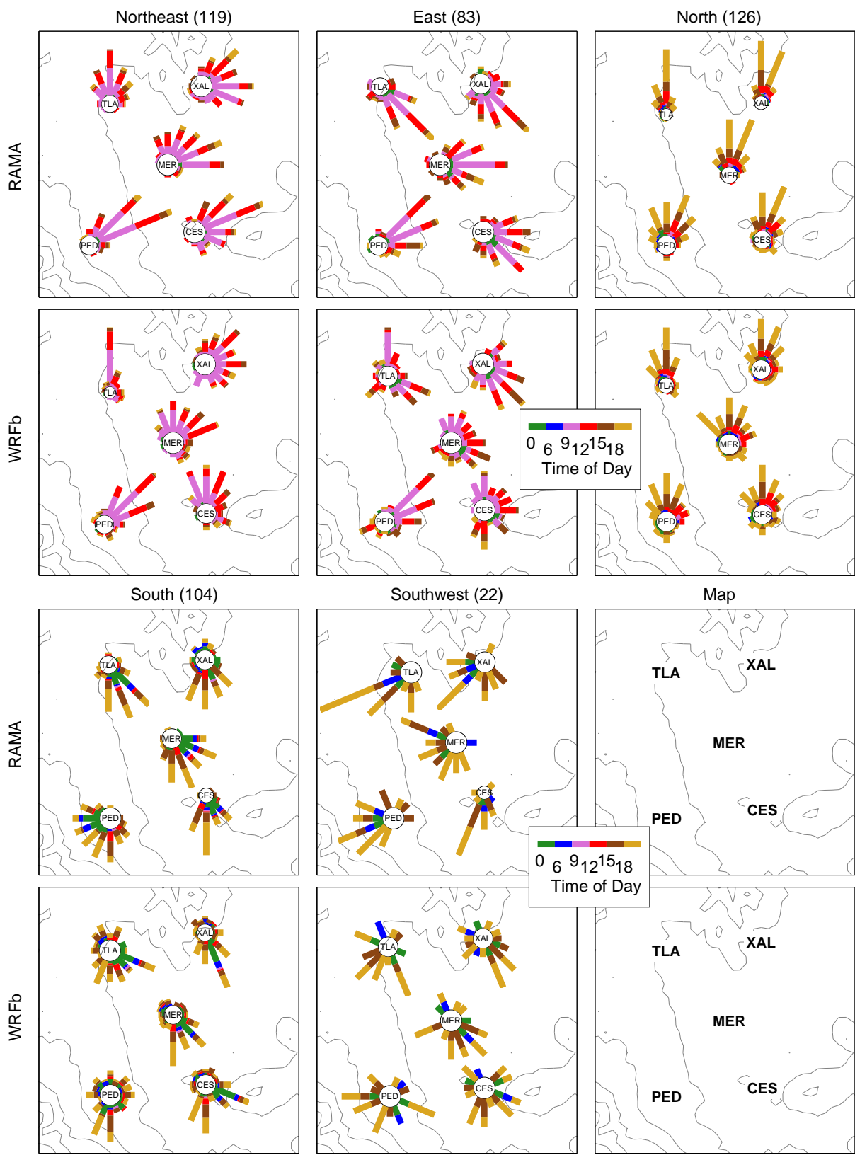
Figure 15: Comparison of surface wind clusters from RAMA measurements and the WRFb case for the north and south flow clusters occurring during MILAGRO. Station data from TLA and XAL (north), MER (centre), PED and CES (south), see Fig. 2 for station locations. Wind rose categories by time of day. Terrain contours every 250 m.
