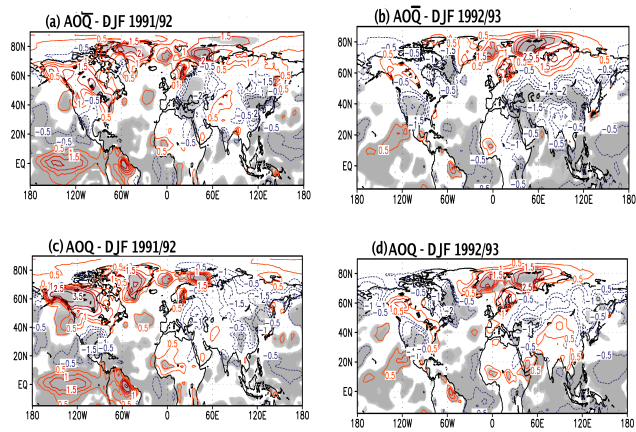
Fig. 6. 2 m temperature anomalies (K) for (a) AO\bar{Q} : DJF 1991/1992 (b) AO\bar{Q} : DJF 1992/1993, when the opposite QBO phase is prescribed; and for (c) AOQ: DJF 1991/1992 and (d) AOQ: DJF 1992/1993, when the observed QBO phase is prescribed. The shading denotes three levels (99%, 95% and 90%) of statistical significance in the order of lighter shading.
