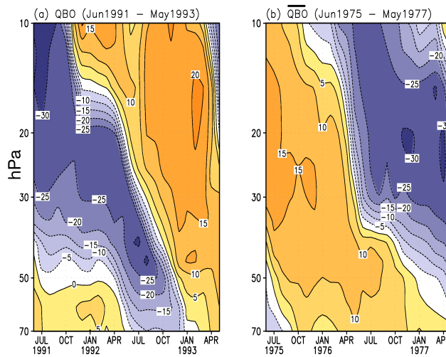
Fig. 1. Zonally averaged observed zonal winds (m/s) at Singapore for (a) June 1991–May 1993 and (b) June 1975–May 1977. Negative values are shaded in colors of blue and are easterlies and the positive values are shaded in colors of yellow and are the westerlies. The contour intervals are 5 m/s.
