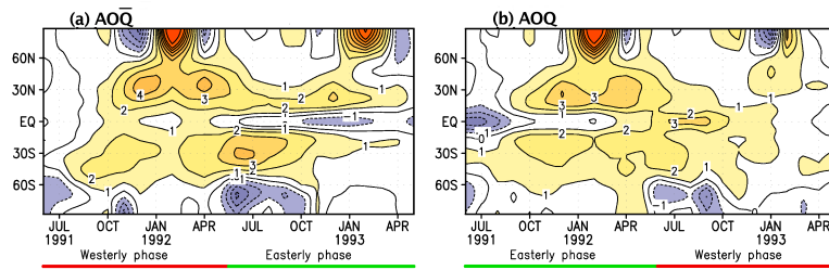
Fig. 4. Zonally averaged lower stratospheric temperature anomalies (K) at 30 hPa for two years following Mt. Pinatubo eruption for (a) AOQ with the opposite QBO phase and (b) AOQ experiment with observed QBO phase. The QBO phases encountered during (a) and (b) are shown by the colored lines.
