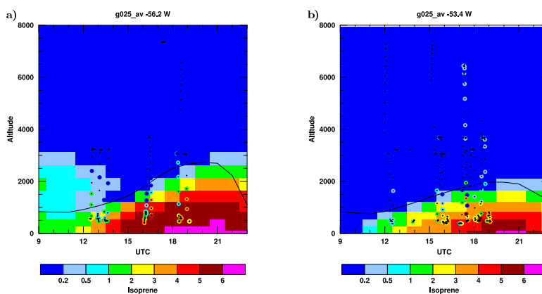
Fig. 3. GABRIEL isoprene measurements (coloured points) superimposed on the modelled diurnal evolution of the October average isoprene mixing ratios from the MIMvK model run ( \text{nmol mol}^{-1} ), along with the model diagnosed mixed layer height (solid line) for the grid cell corresponding with (a) Suriname and (b) French Guyana.
