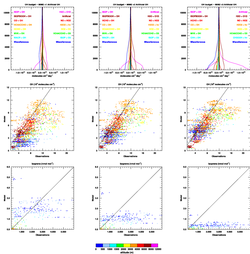
Fig. 7. Effect of progressively adding more artificial OH to the MIM2 mechanism.
