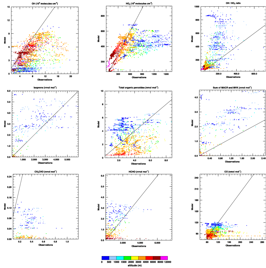
Fig. 4. Model-measurement comparison for several trace species observed during GABRIEL for the MIMvK model run. 6305
