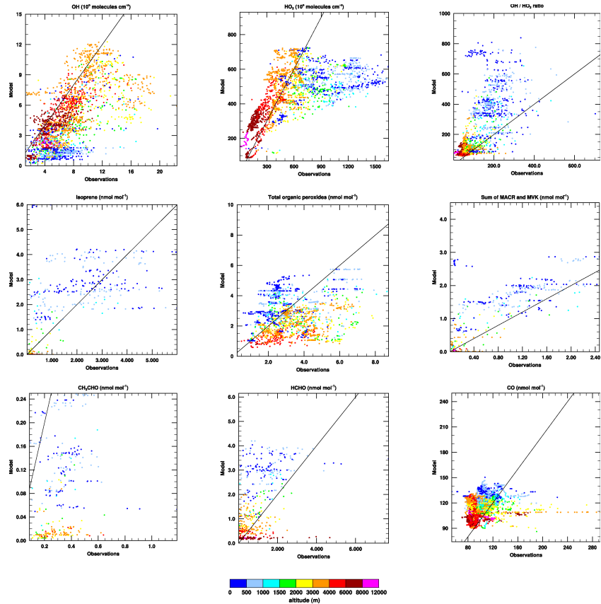
Fig. 5. Model-measurement comparison for several trace species observed during GABRIEL for the MIM2 model run. 6306
