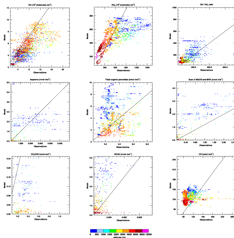
Fig. 9. Model-measurement comparison for several trace species observed during GABRIEL for the run with both artificial OH and a 50% increase in the global isoprene flux. 6310
