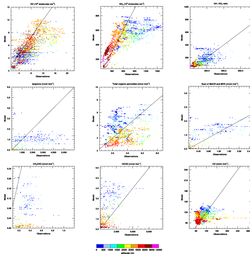
Fig. 8. Model-measurement comparison for several trace species observed during GABRIEL for the run performed with MIM2 and two artificial OH radicals produced from the reaction of HO 2 with peroxides of isoprene. 6309
