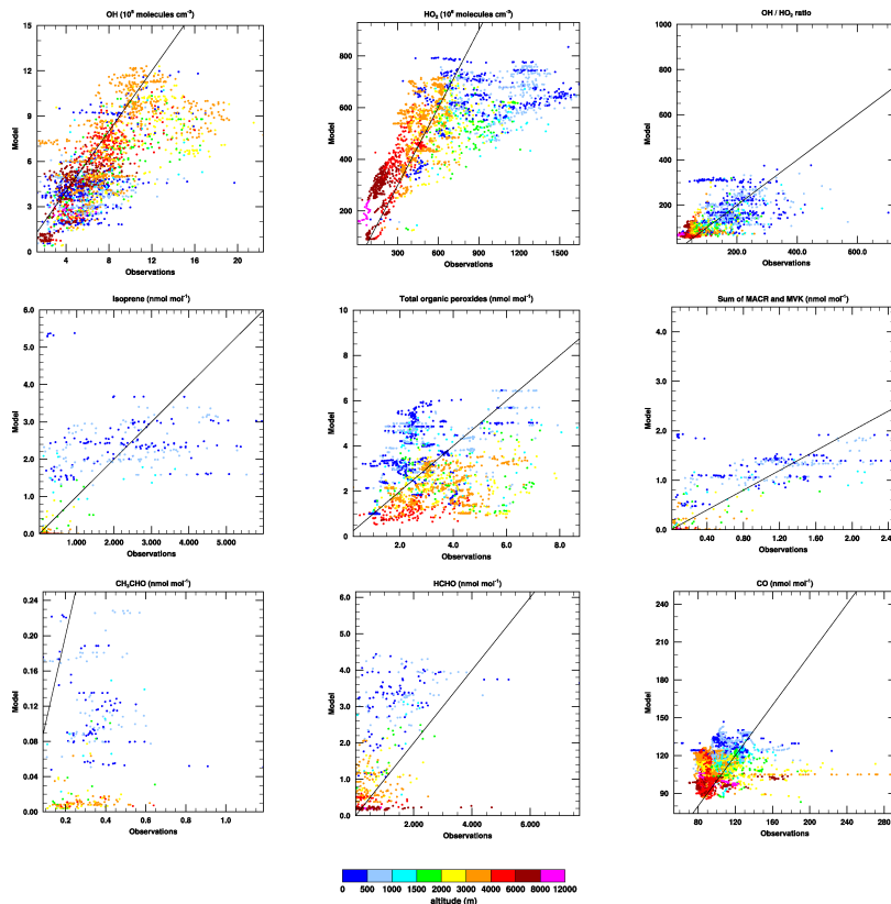
Fig. 10. Model-measurement comparison for several trace species observed during GABRIEL for the run with both artificial OH and the reduced rate constant for isoprene + OH. 6311
