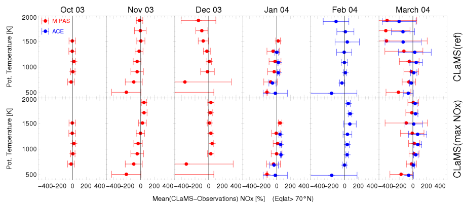
Fig. 5. The mean deviations of the simulated \text{NO}_x mixing ratios from MIPAS observations processed at IMK/IAA (red) and from ACE-FTS observations (blue, from January 2004). The mean deviations are calculated for bins with an altitude range of 200 K potential temperature and for equivalent latitudes poleward of 70^\circ \text{N} . In the columns, the mean deviations from October 2003 until March 2004 are shown. In the top row the results for the reference run and in the bottom row the “max \text{NO}_x ” run are shown. The standard deviation of the mean deviations is indicated by error bars. We note that for February 2004 no \text{NO}_x data from MIPAS processed at IMK/IAA are available. The plot symbols are shifted by a small range in y-direction to distinguish better between MIPAS and ACE-FTS observations.
