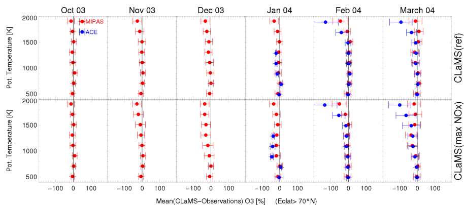
Fig. 6. As Fig. 5, but for ozone.
