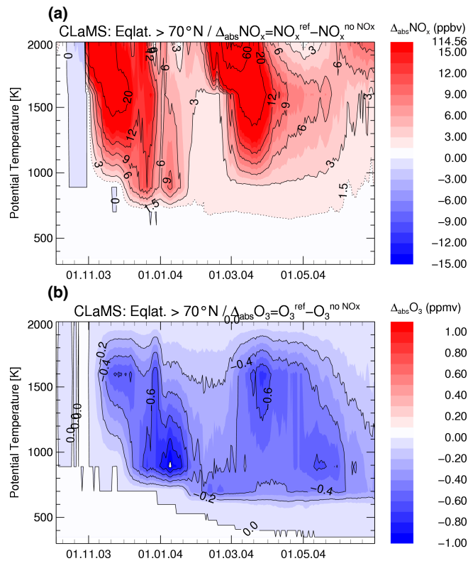
Fig. 8. (a) Additional \text{NO}_x ( \Delta_{\text{abs}}\text{NO}_x ) and (b) ozone reduction \Delta_{\text{abs}}\text{O}_3 poleward of 70°N equivalent latitude due to mesospheric \text{NO}_x intrusions over the course of the winter 2003–2004 for the reference model run.
