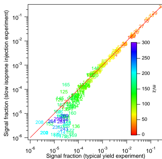
Fig. 9. AMS spectra signal from the slow isoprene injection experiment versus a typical yield experiment. Each mass fragment is normalized by the total signal. The solid red line is the 1:1 line.
