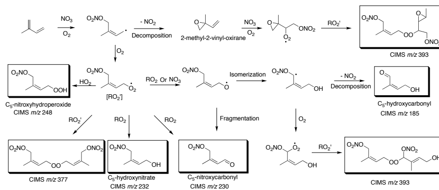
Fig. 11. Proposed mechanisms for the formation of various gas-phase intermediate products observed by CIMS. Multiple structural isomers are possible. In this figure, RO_2' refers to the isoprene peroxy radical (nitroxyperoxy radical), RO_2 refer to a generic peroxy radical.
