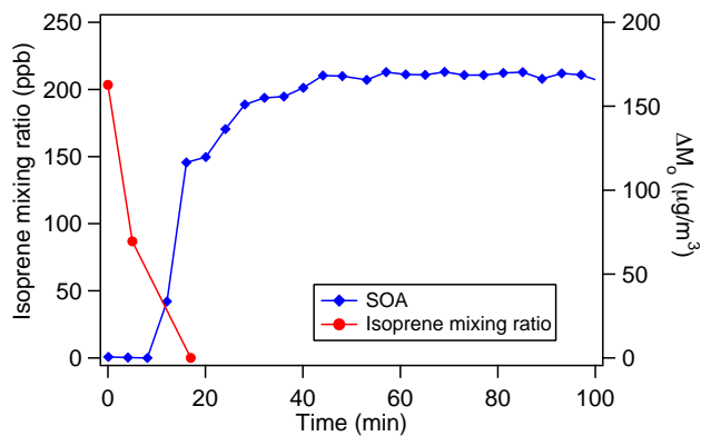
Fig. 2. Reaction profile of the oxidation of an initial mixture containing 203.4 ppb isoprene.
