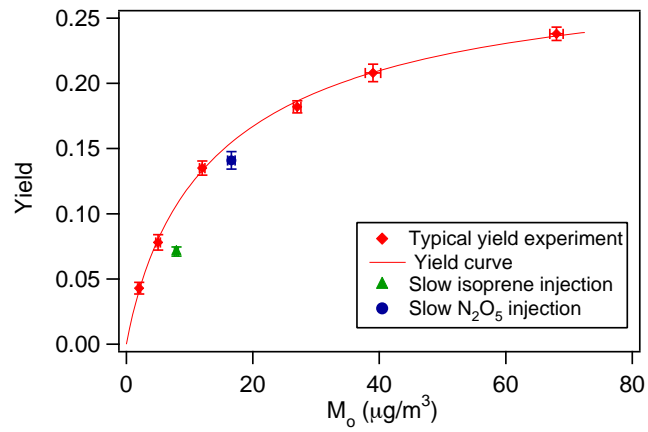
Fig. 3. SOA yield data and yield curve for isoprene- \text{NO}_3 reaction. Also shown are SOA yields from the slow \text{N}_2\text{O}_5 injection experiment and slow isoprene injection experiment.
