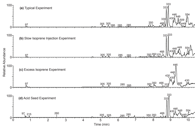
Fig. 10. UPLC/(-)ESI-TOFMS base peak ion chromatograms (BPCs) for the following isoprene- \text{NO}_3 oxidation experiments: (a) 200 ppb isoprene + 1 ppm \text{N}_2\text{O}_5 + seed aerosol generated from 15 mM (\text{NH}_4)_2\text{SO}_4 atomizing solution; (b) 300 ppb isoprene + 1 ppm \text{N}_2\text{O}_5 + seed aerosol generated from 15 mM (\text{NH}_4)_2\text{SO}_4 atomizing solution; (c) 1.2 ppm isoprene + 700 ppb \text{N}_2\text{O}_5 + seed aerosol generated from 15 mM (\text{NH}_4)_2\text{SO}_4 atomizing solution; (d) 200 ppb isoprene + 1 ppm \text{N}_2\text{O}_5 + seed aerosol generated from 30 mM \text{MgSO}_4 +50 mM \text{H}_2\text{SO}_4 atomizing solution. The numbers indicated above the selected chromatographic peaks correspond to the most abundant negative ion, and is either the [\text{M}-\text{H}]^- or [\text{M}-\text{H}+\text{C}_2\text{H}_4\text{O}_2]^- ions.
