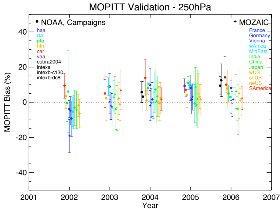
Fig. 6. As Fig. 4, for the 250 hPa retrieval.
