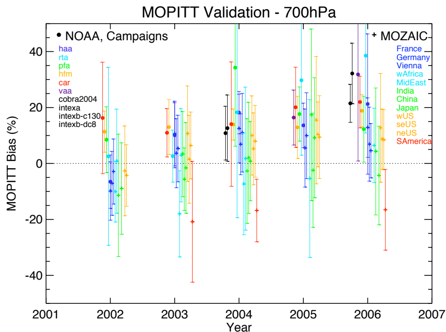
Fig. 5. As Fig. 4, for the 700 hPa retrieval.
