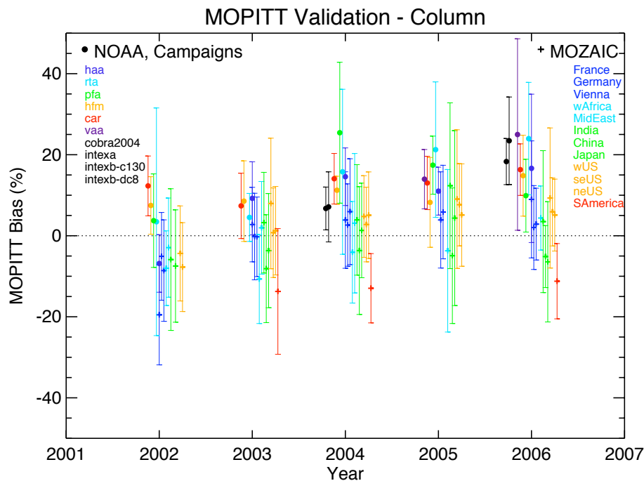
Fig. 4. Bias between MOPITT and aircraft in situ measurements for the column retrieval for each year, sorted by NOAA site, Field Campaign or MOZAIC geographical region. Each symbol and error bar indicates the mean and standard deviation of the biases for each site or region.
