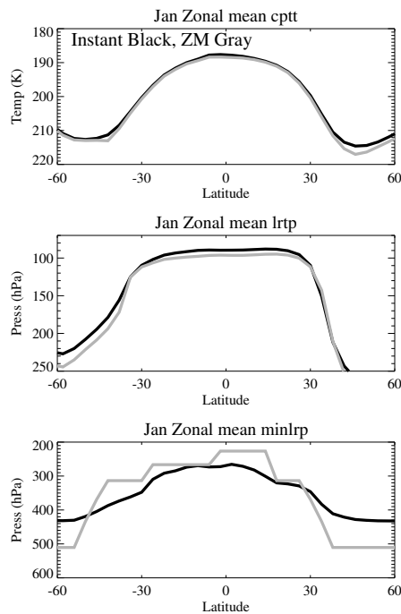
Fig. 1. Comparison between TTL diagnostics calculated using instantaneous 3-D output (Black) and zonal mean monthly output (Gray) for Cold Point tropopause temperature (top), lapse rate tropopause pressure (middle) and lapse rate minimum pressure (bottom).
