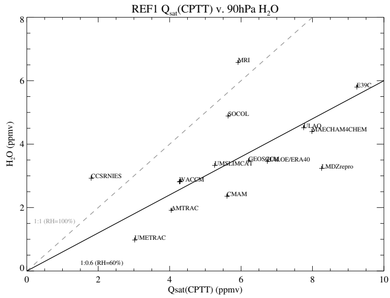
Fig. 16. Scatterplot of Saturation Vapor Mixing Ratio of the Cold Point Tropopause Temperature, Q_{\text{sat}}(\text{CPTT}) and the 90 hPa tropical water vapor mixing ratio for each historical (REF1) run, as well as using ERA40 temperatures and HALOE 100hPa water vapor (ERA40/HALOE). Gray dashed line is 1:1 line (100% RH), Black solid line is 1:0.6 (60% RH).
