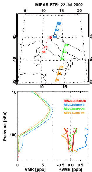
Fig. 7. Comparison of \text{HNO}_3 volume mixing ratio (in ppbv) profiles observed by MIPAS/ENVISAT (solid) and aircraft-based MIPAS-STR measurements (dotted) at mid-latitudes (Forli, Italy) on 22 July 2002. The top panel shows the flight and satellite tangent point tracks for the MIPAS-STR and MIPAS/ENVISAT measured sequences. The numbers indicate the altitudes (in kilometers) of selected flight and satellite tangent points. The bottom panels show the profiles (left) and their differences (right). In the difference panels, the combined noise error is red dotted and the combined total error (without errors from HITRAN) is red solid.
