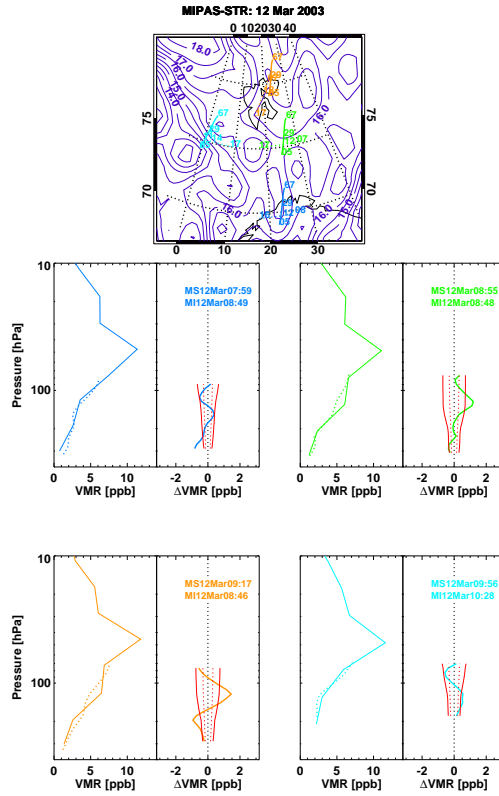
Fig. 10. Same as Fig. 8, but for MIPAS-STR flight at Kiruna, Sweden ( 68^\circ\text{N} , 20^\circ\text{E} ) on 12 March 2003.
