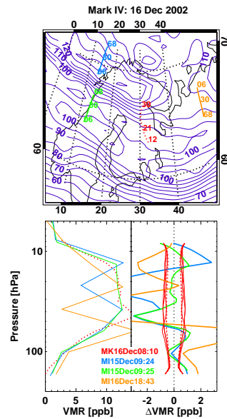
Fig. 16. Comparison of HNO 3 volume mixing ratio (in ppbv) profiles observed by MkIV (red dotted) and MIPAS/ENVISAT (other colors) on 16 December 2002. The top panel shows the balloon flight and satellite tangent point tracks. The numbers indicate the altitudes (in kilometers) of selected tangent points. The bottom panel shows the profiles (left) and their differences (right). In the difference panels, the combined noise error is red dotted and the combined total error (without errors from HITRAN) is red solid. Overlaid violet contour lines are potential vorticity (in 10^{-6} \text{ K m}^2 \text{ kg}^{-1} \text{ s}^{-1} ) at 550 K potential temperature.
