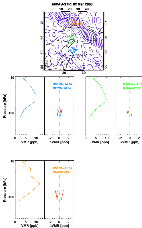
Fig. 9. Same as Fig. 8, but for MIPAS-STR flight at Kiruna, Sweden ( 68^\circ\text{N} , 20^\circ\text{E} ) on 2 March 2003.
