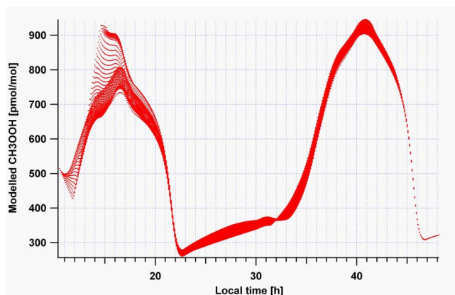
Fig. 13. CH 3 OOH mixing ratios calculated along the 57 different trajectories with the box model (Lagrangian mode, reference run).
