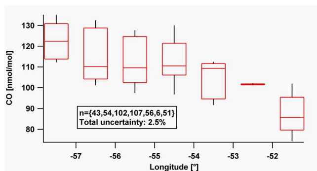
Fig. 2. Longitudinal profile of the CO median mixing ratio in the altitude range 0–1 km a.s.l.; red bar denotes the median; the lower and upper boundary of the red box mark the 25% and 75% percentiles, the bottom and top whisker the 10% and 90% percentiles.
