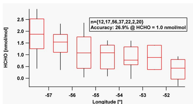
Fig. 4. Longitudinal profile of the HCHO median mixing ratio in the altitude range 0–1 km a.s.l.; as Fig. 2.
