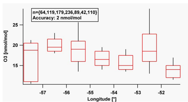
Fig. 3. Longitudinal profile of the O 3 median mixing ratio in the altitude range 0–1 km a.s.l.; as Fig. 2.
