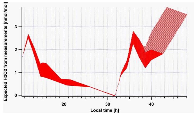
Fig. 10. Expected H 2 O 2 mixing ratios along the 57 different trajectories prescribed by the varying k values. The variation of the mixing ratio as a function of local time arises from the measured longitudinal gradient, the effect of the different starting times of the trajectories and the superimposed diurnal cycle.
