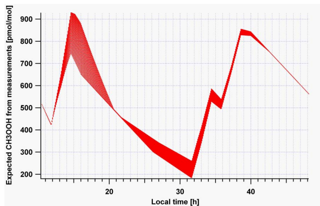
Fig. 12. Expected CH 3 OOH mixing ratios along the 57 different trajectories prescribed by the varying k values. The variation of the mixing ratio as a function of local time arises from the measured longitudinal gradient, the effect of the different starting times of the trajectories and the superimposed diurnal cycle.
