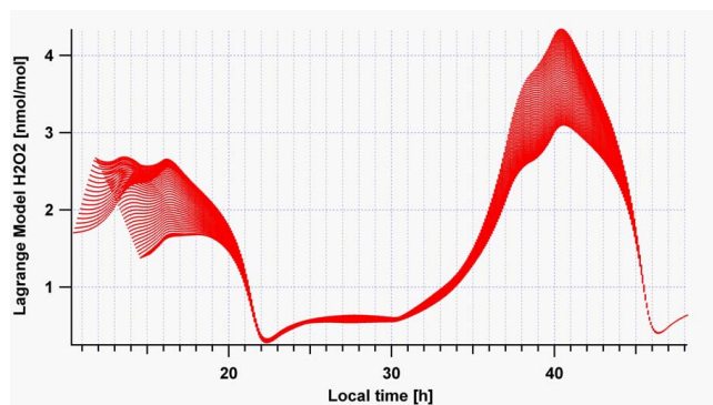
Fig. 11. H 2 O 2 mixing ratios calculated along the 57 different trajectories with the box model (Lagrangian mode, reference run).
