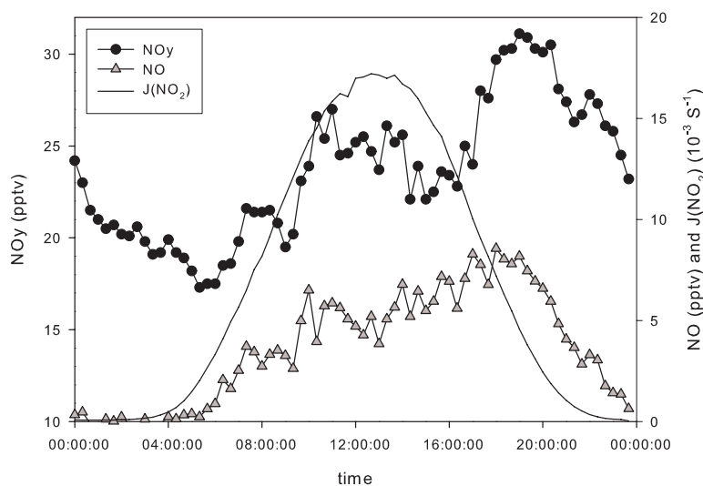
Fig. 7. Diurnal variation in \text{NO}_y , \text{NO} and \text{J-NO}_2 measured at Neumayer Station, Antarctica, 1997, (Weller et al., 1999).
