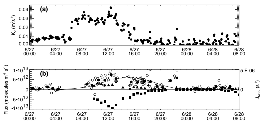
Fig. 4. (a) Eddy diffusivity measurements and (b) calculated fluxes (flux-gradient approach) during 27–28 June at Summit, Greenland. circles = NO x , triangles = HONO, squares = HNO 3 , solid line = J(NO 3 ). Positive values indicate an upward flux. (Reprinted from Honrath et al., Vertical fluxes of NO x , HONO and HNO 3 above the snowpack at Summit, Greenland, Atmospheric Environment, 36, 2629–2640, 2002, with permission from Elsevier).
