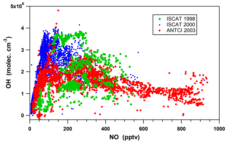
Fig. 9. OH versus NO at South Pole.
