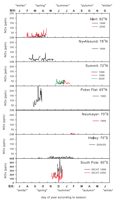
Fig. 6. As for Fig. 5, but for NO x measurements – References as for Fig. 5. South Pole NO x are based on calculated NO 2 values and measured NO values.
