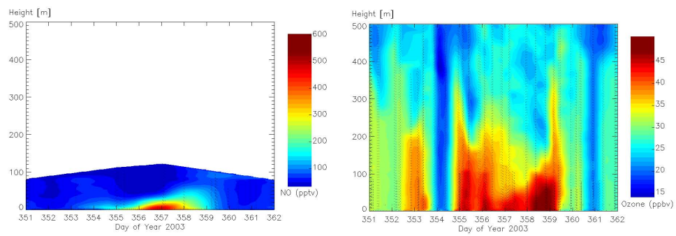
Fig. 11. Comparison of the vertical distribution of NO (left) and ozone (right) during Dec. 2003 at South Pole. These data are from concurrent vertical profile measurements of NO and ozone using a tethered balloon. (Figures adapted from Helmig et al., 2007a, 2007e).
