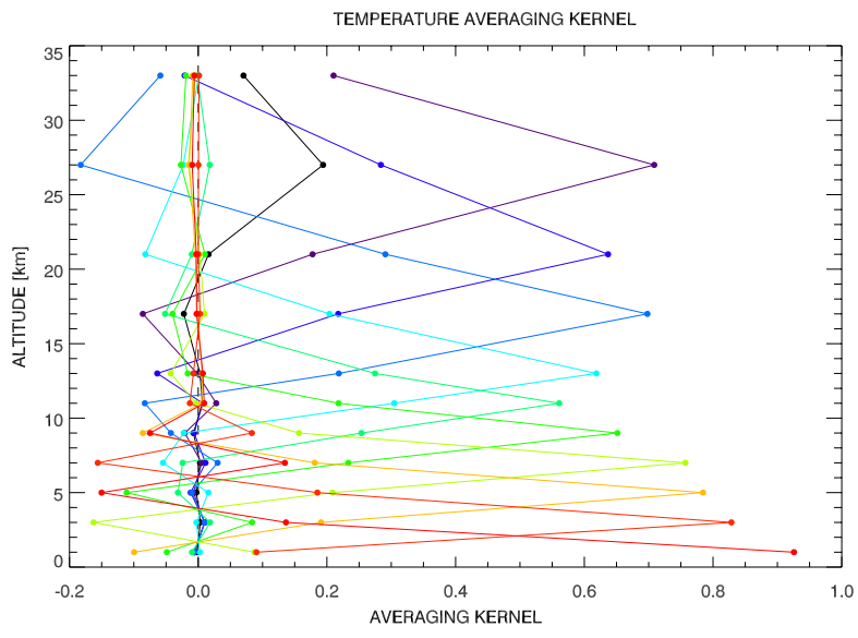
Fig. 3. Averaging kernels for T.
