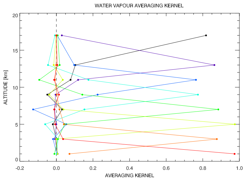
Fig. 4. Averaging kernels for water vapour.
