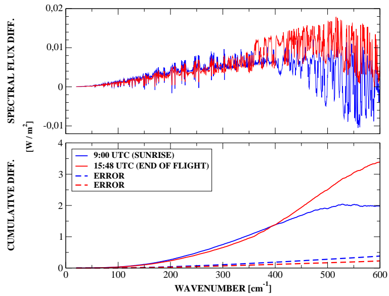
Fig. 9. Difference between the spectral fluxes calculated for the fitted and ECMWF water vapour and temperature profiles. In the figure, the results for 2 sequence measurements are reported as a function of wavenumber (top panel). The cumulative integral is shown in the bottom panel.
