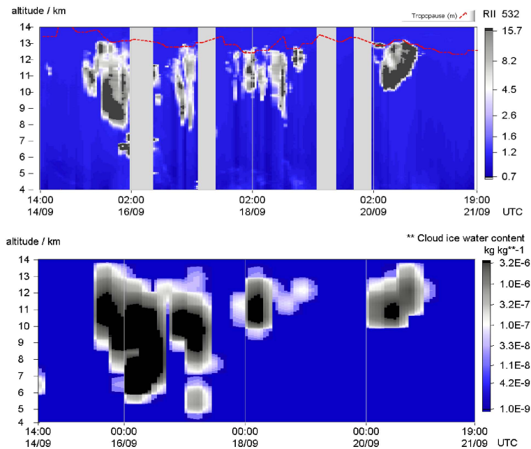
Fig. 6. The upper plot shows lidar observations of cirrus clouds in term of the backscatter ratio at 532 nm for one week in September 2003. The lower plot shows the corresponding cloud ice water content at the nearest gridpoint to Lindenberg (52°, 14°) of opECMWF for the same time period.
