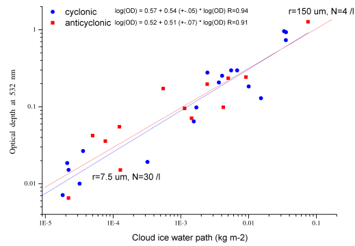
Fig. 7. Comparison of the observed total cirrus cloud optical depth determined from lidar observations with the Ice Water Path of the nearest grid-point of the opECMWF data for August and Spetember 2003.
