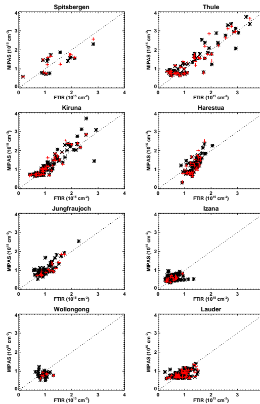
Fig. 14. Scatterplots between MIPAS and FTIR daily mean column amounts for the collocation criterion \Delta d_{\max}=800 km, \Delta t_{\max}=8 h, and \Delta \rho v_{\max}=3 \times 10^{-6} \text{ Km}^2 \text{ kg}^{-1} \text{ s}^{-1} at 475 K (black stars) and \Delta d_{\max}=400 km, \Delta t_{\max}=4 h, and \Delta \rho v_{\max}=3 \times 10^{-6} \text{ Km}^2 \text{ kg}^{-1} \text{ s}^{-1} at 475 K (red crosses).
