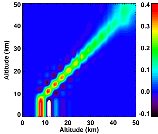
Fig. 1. Averaging kernel of \text{ClONO}_2 retrieval from MIPAS limb-scan on 24 September 2002, 22:07 UTC at 46.1^\circ \text{N}/0.6^\circ \text{E} (Best coincidence with MIPAS-B: Table 3 and Fig. 2).
