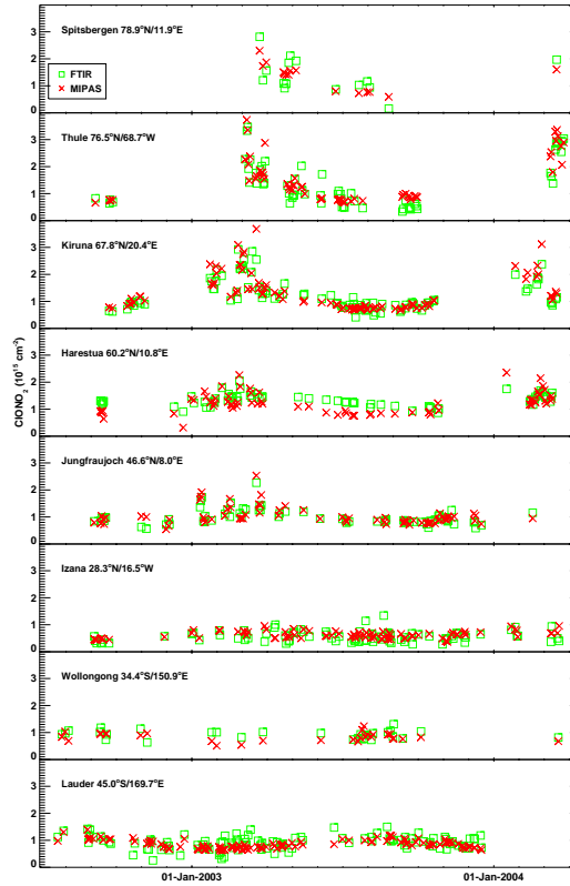
Fig. 13. Comparison between MIPAS (red) and FTIR (green) daily mean column amounts versus time for the collocation criterion \Delta d_{\max}=800 km, \Delta t_{\max}=8 h, and \Delta \rho v_{\max}=3 \times 10^{-6} \text{ Km}^2 \text{ kg}^{-1} \text{ s}^{-1} at 475 K.
