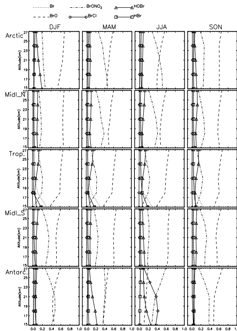
Fig. 8. Partitioning of bromine species as calculated by the 1-D photochemical model. The model was constrained by SCIAMACHY \text{NO}_2 measurements. Calculations were performed for the four seasons December/January/February (DJF), March/April/May (MAM), June/July/August (JJA) and September/October/November (SON) and five latitude bands: Arctic (north of 60^\circ \text{N} ), northern hemisphere mid-latitudes ( 30^\circ \text{N} – 60^\circ \text{N} ), tropics ( 30^\circ \text{S} – 30^\circ \text{N} ), southern hemisphere mid-latitudes ( 30^\circ \text{S} – 60^\circ \text{S} ), and Antarctic (south of 60^\circ \text{S} ).
