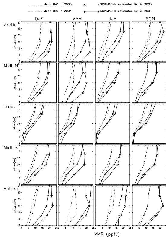
Fig. 11. Seasonal, zonal mean BrO VMRs for the two years 2003 and 2004 along with estimated \text{Br}_y for the same period.
