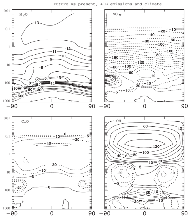
Fig. 22. Changes in water (tenths ppmv, top left), \text{NO}_x (tens pptv, top right), ClO (tens pptv, bottom left) and OH ( 10^4 molecules/ \text{cm}^3 bottom right) between the 2100 A1B composition plus climate run and the present-day simulation.
