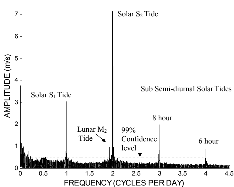
Fig. 1. (a) Lomb-Scargle analysis of zonal horizontal wind data over an interval of 17 years (1988–2005) from the UK meteor radar.
