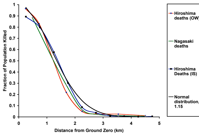
Fig. 2. The fatality curves from Hiroshima ((OW)-Oughertson and Warren, 1956; (IS) Ishikawa and Swain, 1981) and Nagasaki (Oughertson and Warren, 1956), and a normal distribution fit to the Hiroshima data from Ishikawa and Swain (1981) with a standard deviation \sigma=1.15 .
