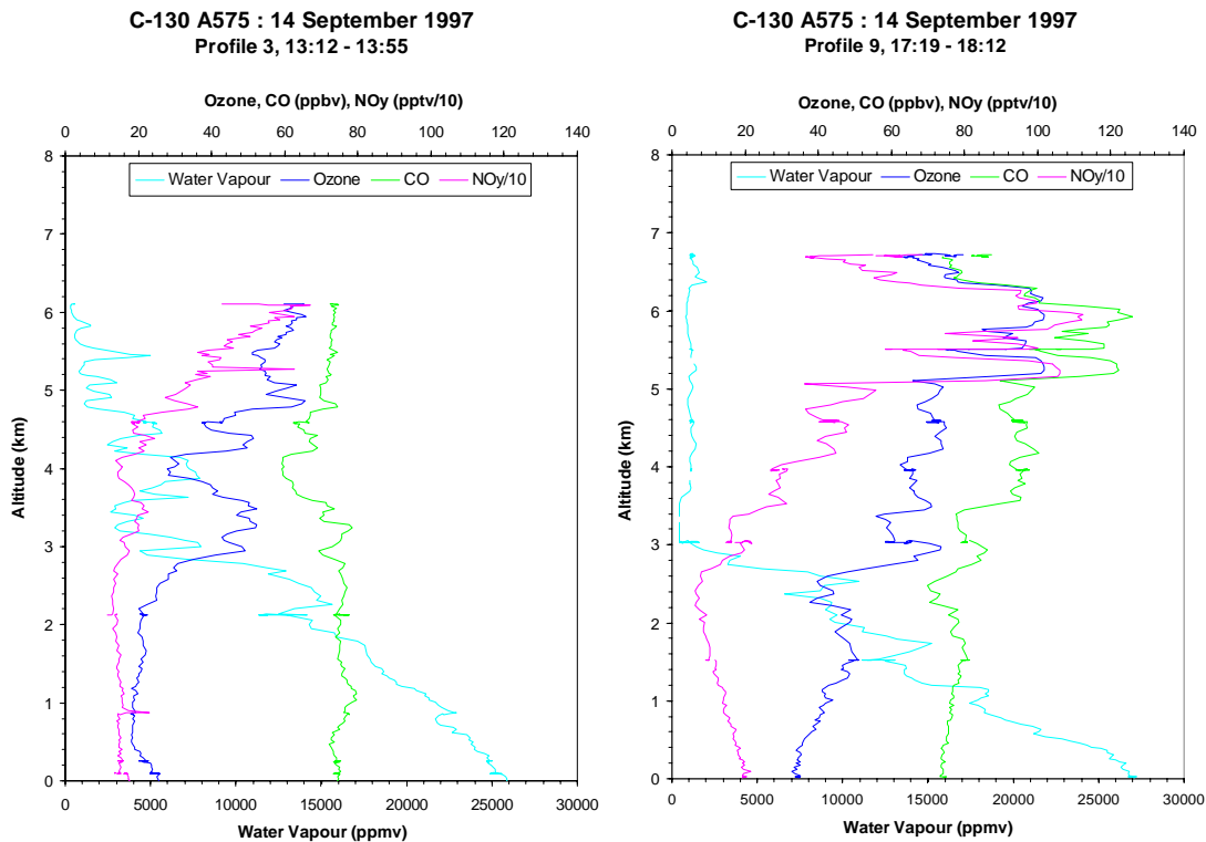
Fig. 4. Vertical profiles of ozone, CO, NOy and water vapour obtained in Flight A575 on 14 September 1997 outside (left hand panel) and inside (right hand panel) the influence of the hurricane (see Fig. 3 for identification of profile numbers).
