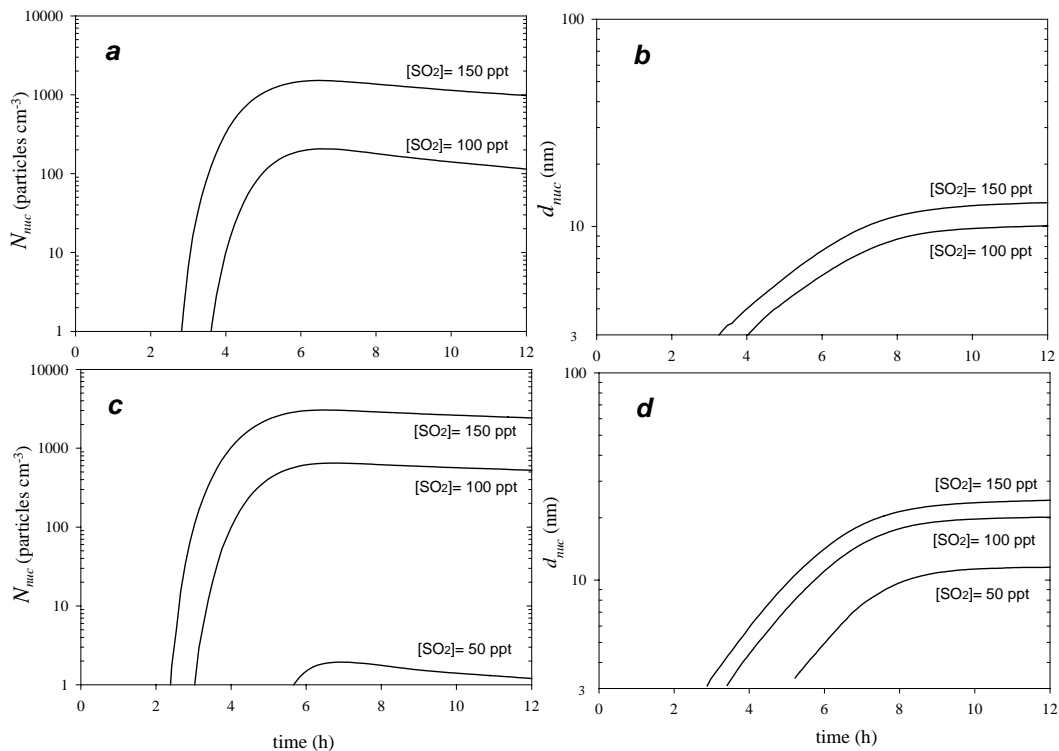
Fig. 5. Time evolution of the number concentration of detectable ( >3 nm) secondary particles N_{nuc} ((a) and (c)) and the mean diameter of the particles d_{nuc} ((b) and (d)). The parameter P_{max} was set equal to 1.6 \times 10^5 \text{ cm}^{-3} \text{ s}^{-1} (top) and 8 \times 10^4 \text{ cm}^{-3} \text{ s}^{-1} (bottom). The values of the other input parameters were chosen as in Fig. 3.
