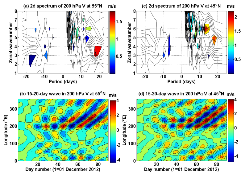
Figure 1. (a) Space–time spectra of ERA-interim meridional winds at 200 hPa at 55 and 45° N and (b) 15–20 day filtered ERA-interim meridional winds at 55 and 45° N for the period December 2012–February 2013.
