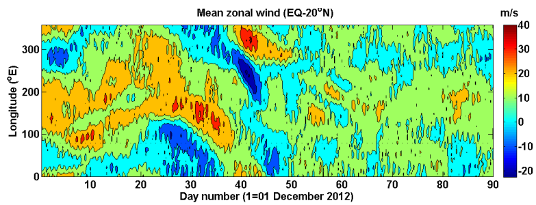
Figure 5. Time–longitude cross section of ERA-interim zonal wind at 200 hPa averaged for the latitudes 0–20° N.
