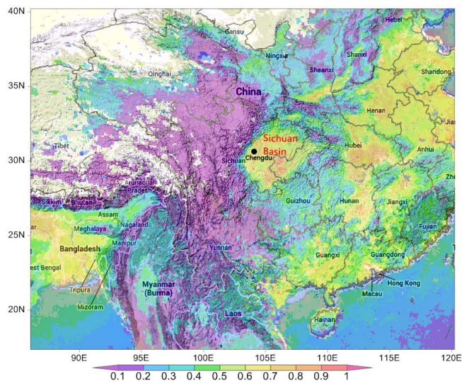
Fig. 1. Sampling location (30.65° N, 104.03° E) in Chengdu on a regional map superimposed with spatial distribution of annual mean aerosol optical depth (AOD) retrieved from MODIS satellite remote sensing in 2011.
