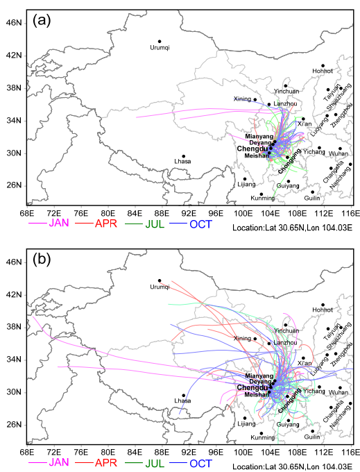
Fig. 10. Analytical results of the 48 h air mass back trajectories at 500 m (a) and 1500 m (b) elevation during the sampling periods, which were run four times per day.
