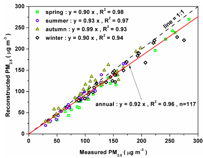
Fig. 4. Correlation between reconstructed and measured PM_{2.5} mass concentrations in four seasons. Also shown are the linear regression lines with regression equations.
