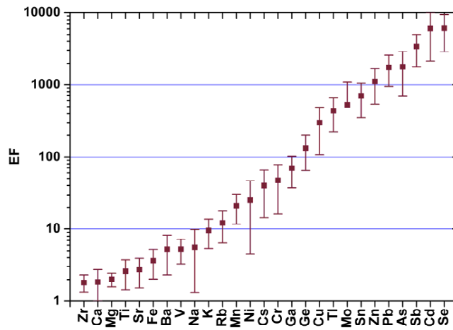
Fig. 3. Enrichment factors of trace elements.
