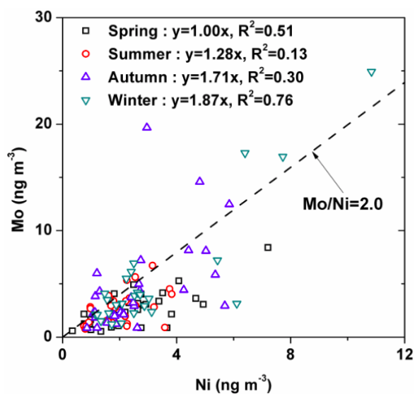
Fig. 9. Scatter plots of Mo and Ni in four seasons.
