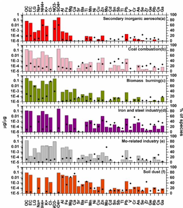
Fig. 6. Six source profiles (bars) resolved from the PMF model (in unit \mu\text{g}/\mu\text{g}^{-1} ). Also shown is contribution percentages (black dots) from each source factor (in unit %).
