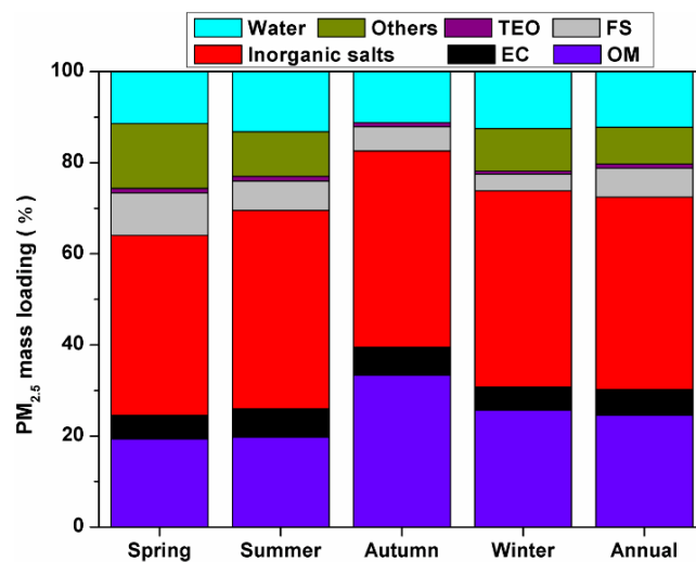
Fig. 5. Chemical mass closures of PM 2.5 mass concentrations in four seasons. The major chemical components include inorganic salts, organic matter (OM), elemental carbon (EC), fine soil (FS), trace element oxides (TEO), water content, as well as others that were unidentified.
