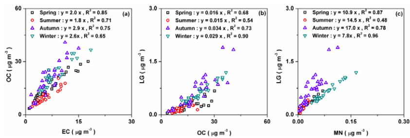
Fig. 2. Scatter plots of OC vs. EC (a), LG vs. OC (b) and LG vs. MN (c) in four seasons. Also shown are the linear regression lines with regression equations.
