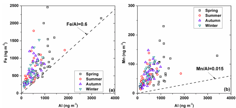
Fig. 8. Scatter plots of Fe vs. Al and Mn vs. Al in PM_{2.5} of Chengdu.
