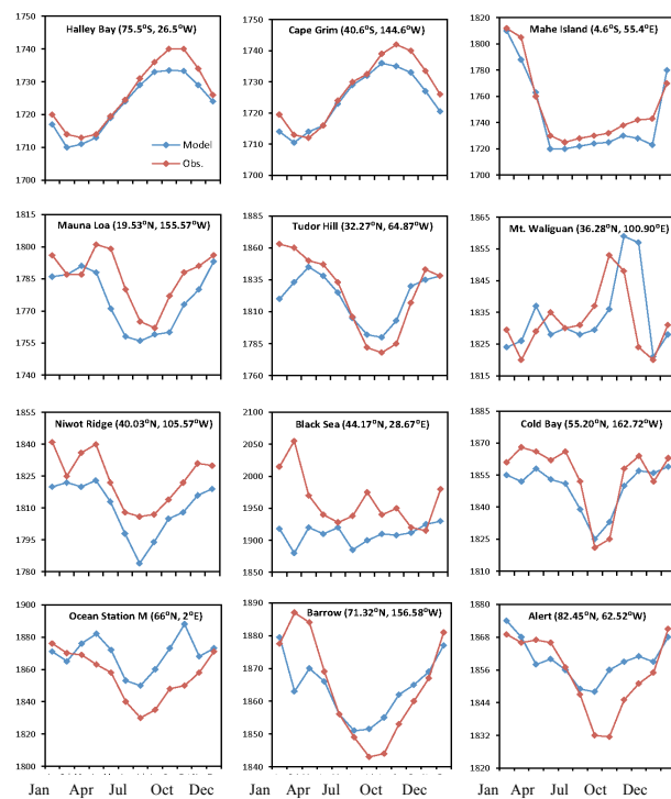
Fig. 7. Model-observation comparison of surface methane mixing ratios (in \text{nmol mol}^{-1} ) at selected sites. Observations are averaged between 1986 and 2006. The model data is the monthly average of output of four years in its equilibrium state.
