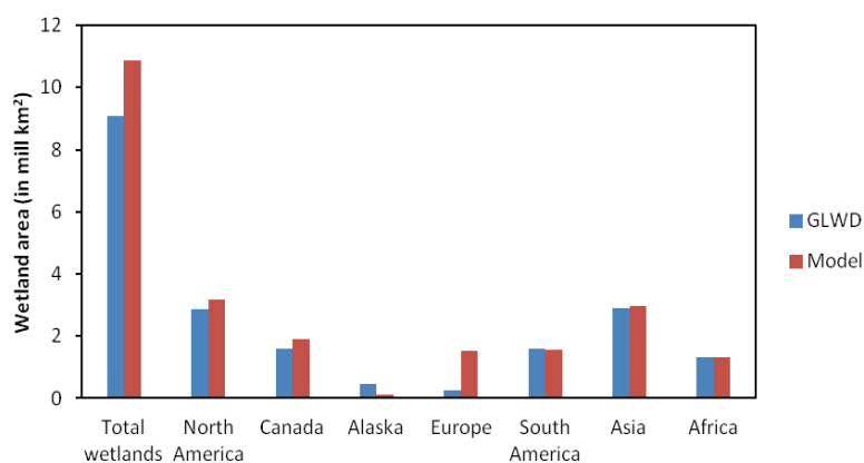
Fig. 2. Regionally aggregated wetland areas from this study compared to the Global Lake and Wetland Database (GLWD) of Lehner and Döll (2004).
