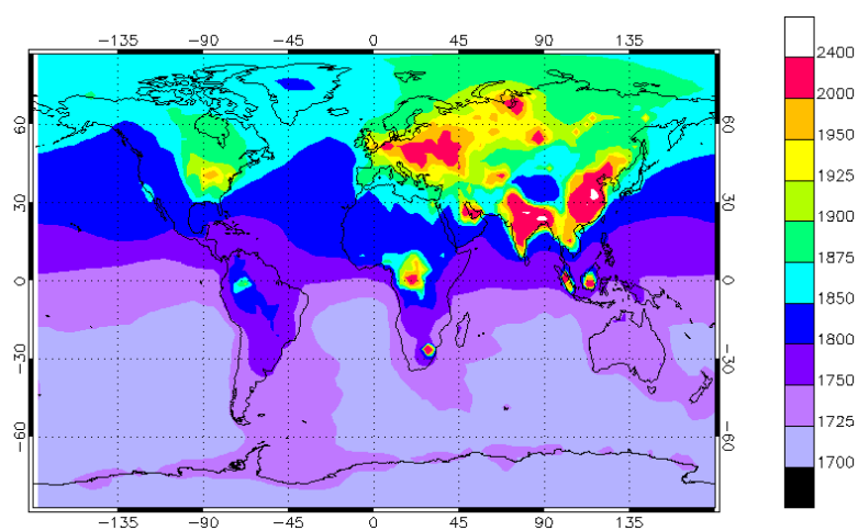
Fig. 6. Annual mean present day surface methane distribution (in nmolmol -1 ) from the ECHAM5 atmospheric model simulation.
