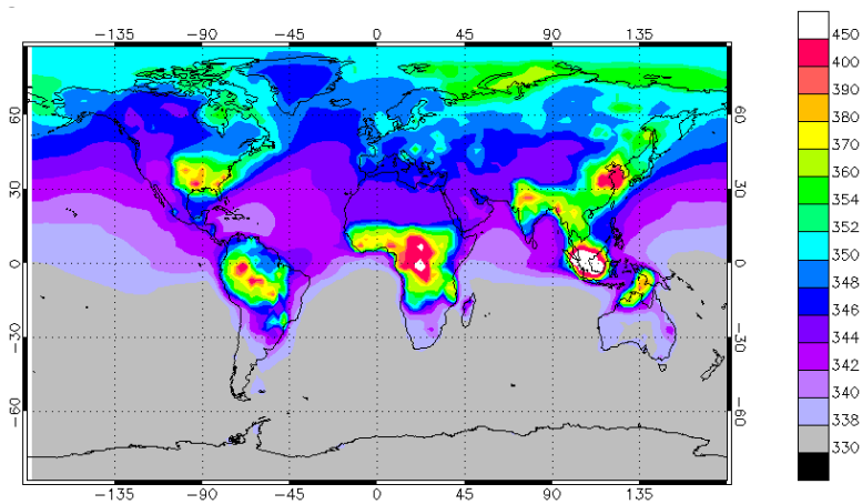
Fig. 10. The spatial distribution of the annual mean surface methane mixing ratio (in \text{nmol mol}^{-1} ) for LGM from ECHAM5 atmospheric model simulation.
