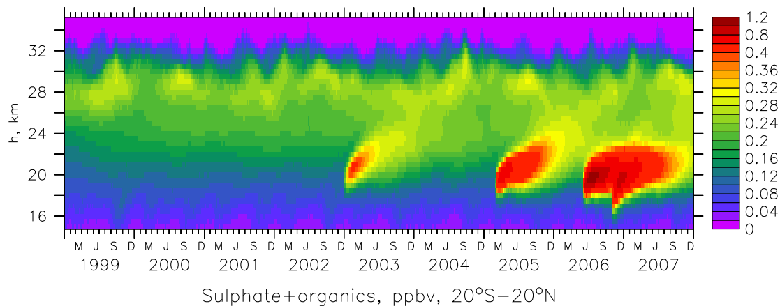
Fig. 3. Improved Figure 8b, sulphate and organics.
