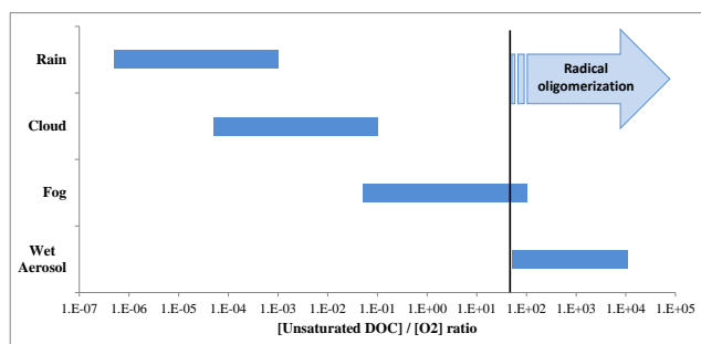
Fig. 12: Estimated ranges of the ratios of unsaturated dissolved organic carbon concentration to oxygen concentration (in M M^{-1} ) in atmospheric waters. The straight lines delimit the values for which radical oligomerization dominates over O_2 addition, as determined by the present work (see text).
