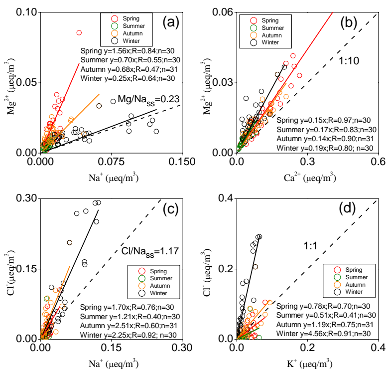
Fig. 4. Correlations between certain cations and anions: (a) Mg^{2+} versus Na^+ , (b) Mg^{2+} versus Ca^{2+} , (c) Cl^- versus Na^+ , and Cl^- versus K^+ . Four seasons are considered and represented by different color symbols. Linear regression equations are also given. In panels (a) and (c), the dashed lines indicate the Mg/Na and Cl/Na equivalent concentration ratios in seawater (sea salt), respectively.
