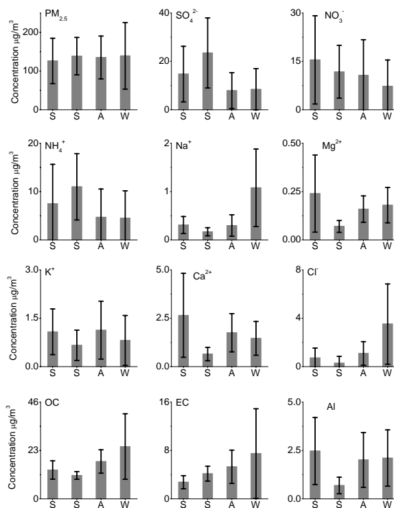
Fig. 2. Seasonal variations of PM 2.5 mass concentration and associated species, including SO 4 2- , NO 3 - , NH 4 + , Na + , Mg 2+ , K + , Ca 2 + , Cl - , OC, EC, and Al concentrations. Shown here are the mean and one standard deviation for each bar.
