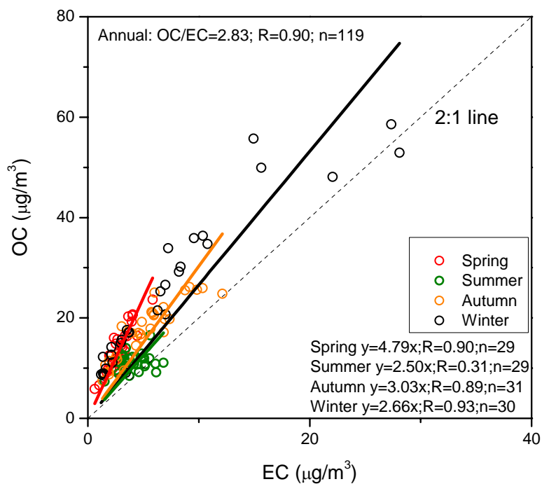
Fig. 3. Scatter plot showing the correlation between OC (y-axis) and EC (x-axis) in PM_{2.5} collected from Beijing. Different symbols denote the four seasons. Linear regression equations are given in the annual and seasonal cases.
