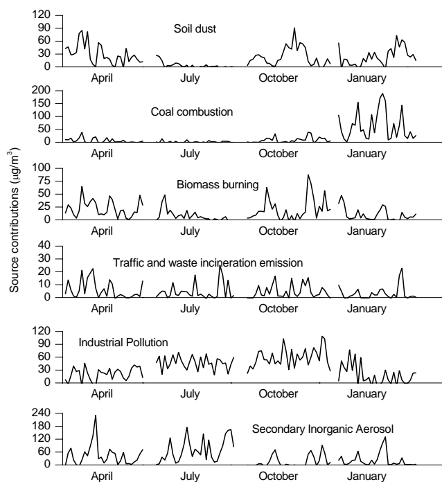
Fig. 9. Time-series of daily contributions from each identified source, including soil dust, coal combustion, biomass burning, traffic and waste incineration emission, industrial pollution, and secondary inorganic aerosol (from the upper to the lower panels) during the study period between April 2009 and January 2010.
