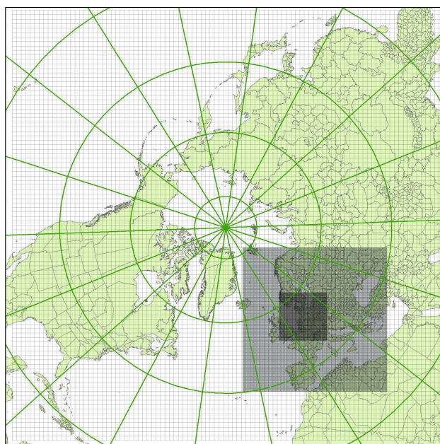
Fig. 2. The DEHM model domain (polar stereographic projection) with two nests. The mother domain covers the Northern Hemisphere with a resolution of 150\text{ km} \times 150\text{ km} . The two nested domains included have resolution of 50\text{ km} \times 50\text{ km} (domain 2) and 16.67\text{ km} \times 16.67\text{ km} (domain 3), respectively.
