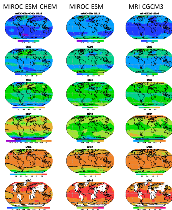
Fig. A2b. Temperature trend (°C decade -1 ) distribution in the selected CMIP5 model. Left: MIROC-ESM-CHEM; middle: MIROC-ESM; right: MRI-CGCM3.
