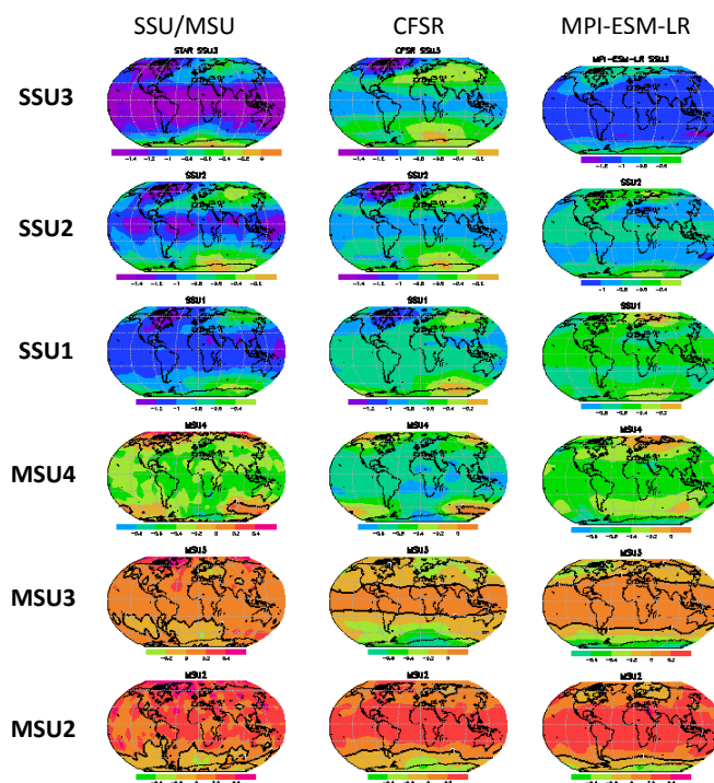
Fig. 5. Temperature trends ( ^{\circ}\text{C decade}^{-1} ) distribution in SSU/MSU observation (left panel), a reanalysis (middle panel) and a selected CMIP5 model (right panel).
