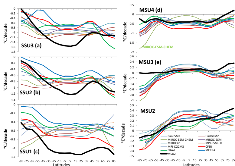
Fig. 7. Temperature trends ( ^{\circ}\text{C}/\text{decade}^{-1} ) change with latitudes (a) SSU3, (b) SSU2, (c) SSU1, (d) MSU4, (e) MSU3, (f) MSU2. Note SSU1 ~ SSU3 and MSU2 ~ MSU4 represent the layer of the SSU and MSU observations. Note SSU1 ~ 3 and MSU2 ~ 4 represent the SSU/MSU observational layers.
