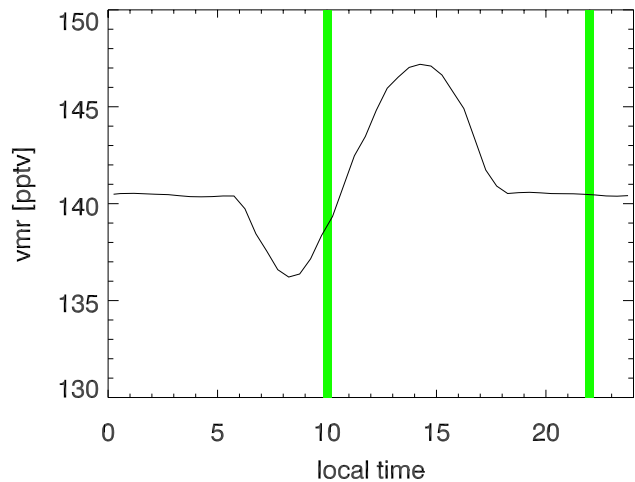
Fig. 11. Diurnal cycle of \text{H}_2\text{O}_2 vmr in KASIMA in dependency of local time in 30 km; The vertical lines mark MIPAS measurement times.
