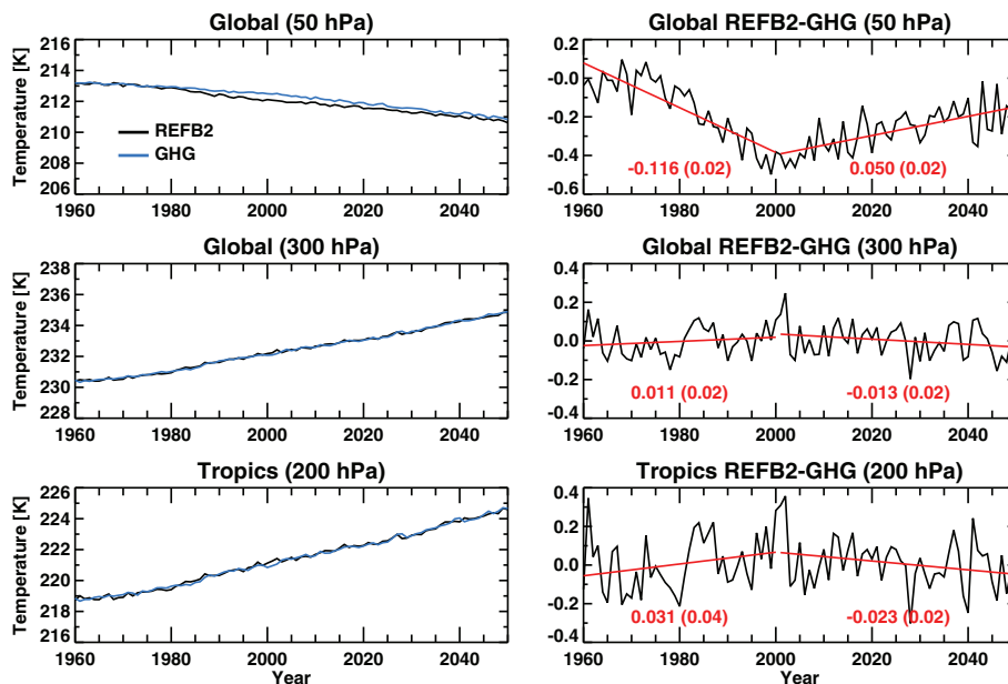
Fig. 3. Annual mean temperature time series: global average at 50 hPa (top), global average at 300 hPa (middle) and tropical average ( 20^{\circ} S– 20^{\circ} N) at 200 hPa (bottom). Left panels show REF-B2 (black) and GHG (blue); right panels show REF-B2 minus GHG (black) and the corresponding linear trends and 95 % uncertainties (in brackets) for 1960–2000 and 2001–2050 in \text{K decade}^{-1} .
