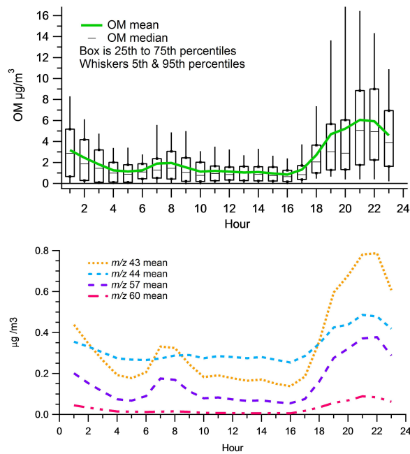
Fig. 2. (a) Box plot of AMS OM ( \mu\text{g m}^{-3} ) by hour, and (b) average concentrations of selected m/z (43, 44, 57, and 60) by hour.
