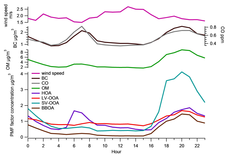
Fig. 7. PMF factor contributions, OM, BC, CO and wind speed averaged by hour.
