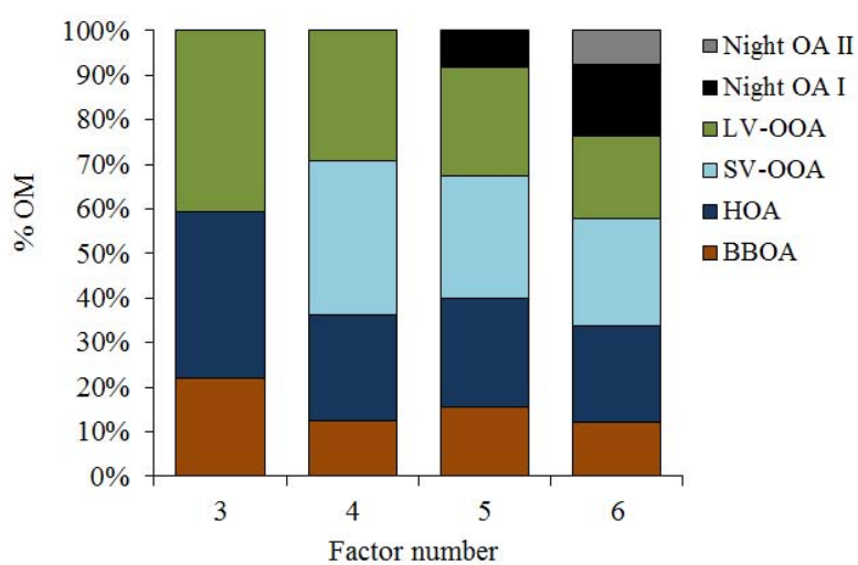
Fig. 5. Summary of OM apportioned by factor number.
