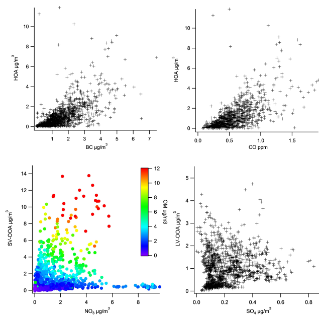
Fig. 9. Scatter plot comparisons of PMF factor contributions for: (a) HOA and BC; (b) HOA and CO; (c) SV-OOA and nitrate; and d) LV-OOA and sulfate.
