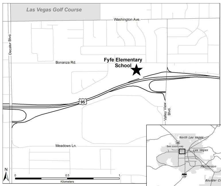
Fig. 1. Location of Fyfe Elementary School in Las Vegas, Nevada.
