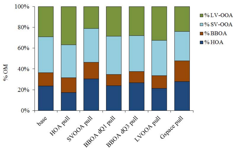
Fig. 11. Attribution of OM with four factors for base run, with ratio of m/z 43/44 in the SV-OOA profile pulled toward the 5-h aged diesel profile; ratio of m/z 41/43 in the HOA profile pulled toward the diesel exhaust profile; ratio of m/z 60/91 in the BBOA profile pulled toward the oak-flame source profile; m/z 44 in LV-OOA profile pulled up maximally; and edge points on the HOA/LV-OOA G-space plot pulled down to the y- and x-axes.
