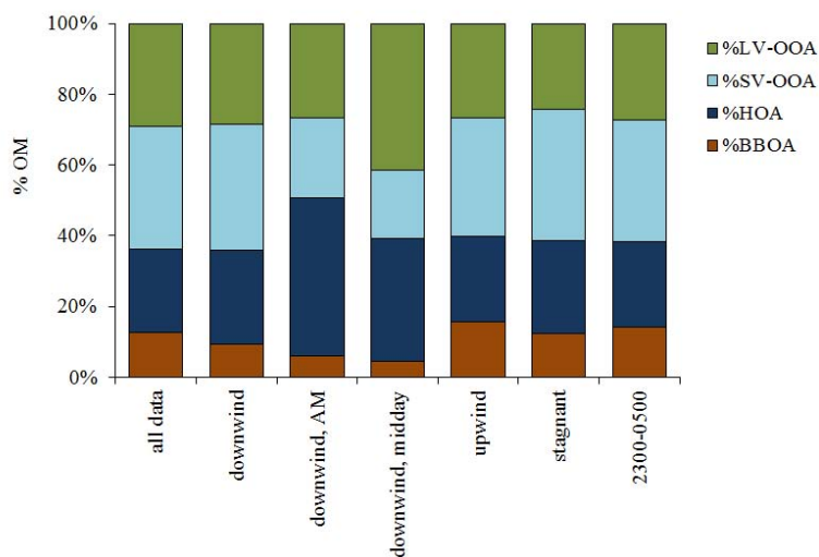
Fig. 10. Attribution of OM by factor in the four-factor solution over all data, during downwind conditions only, during downwind conditions between 05:00 and 09:00 LST only, during upwind conditions only, during stagnant conditions, and during 23:00–05:00 LST only.
