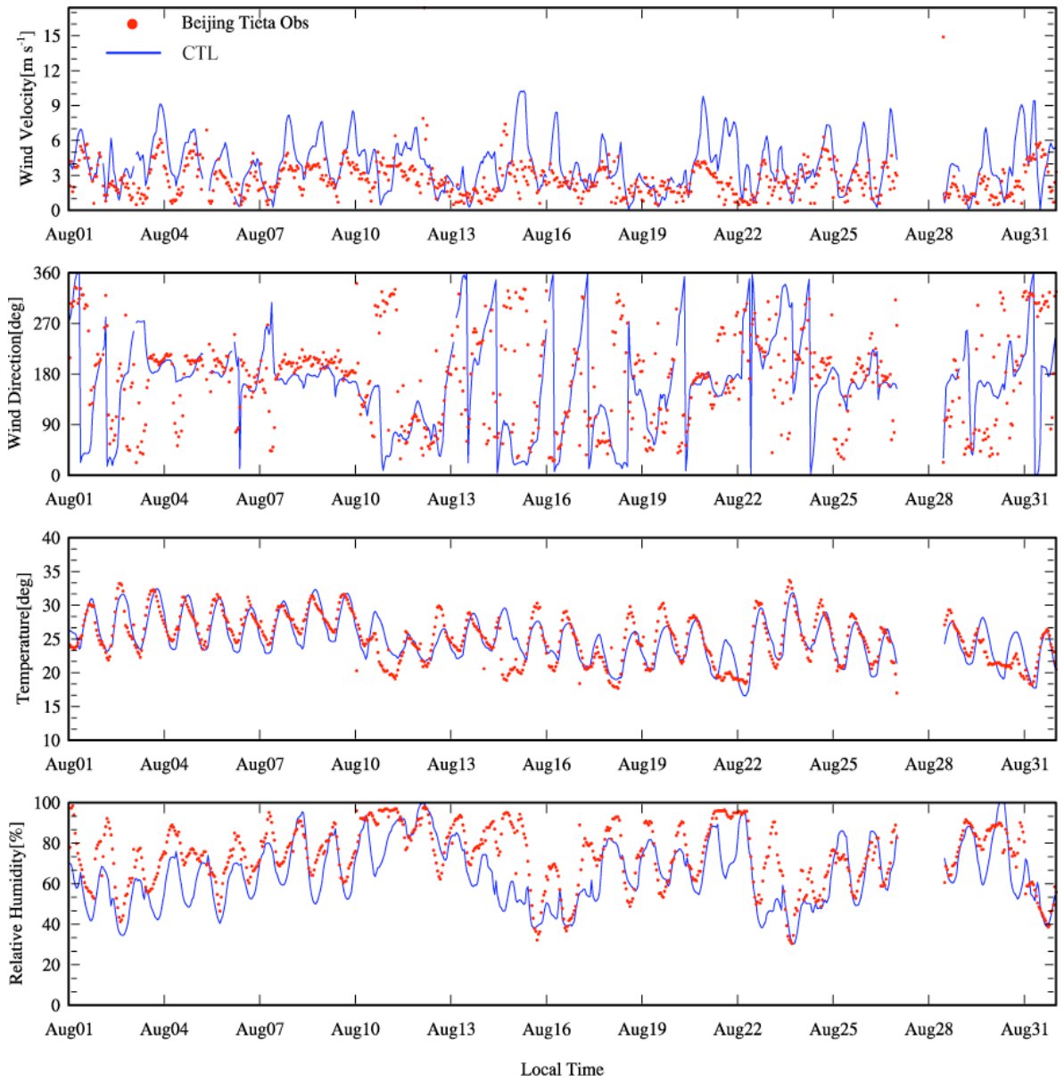
Figure S1. Comparison of model outputs at ~100 m (model level 4 from bottom) with observed hourly wind speed, wind direction, temperature and relative humidity at the seventh platform (100 m) of the 325-m meteorological tower (116.4°E, 40°N) at the Institute of Atmospheric Physics in Beijing for August 2008.
