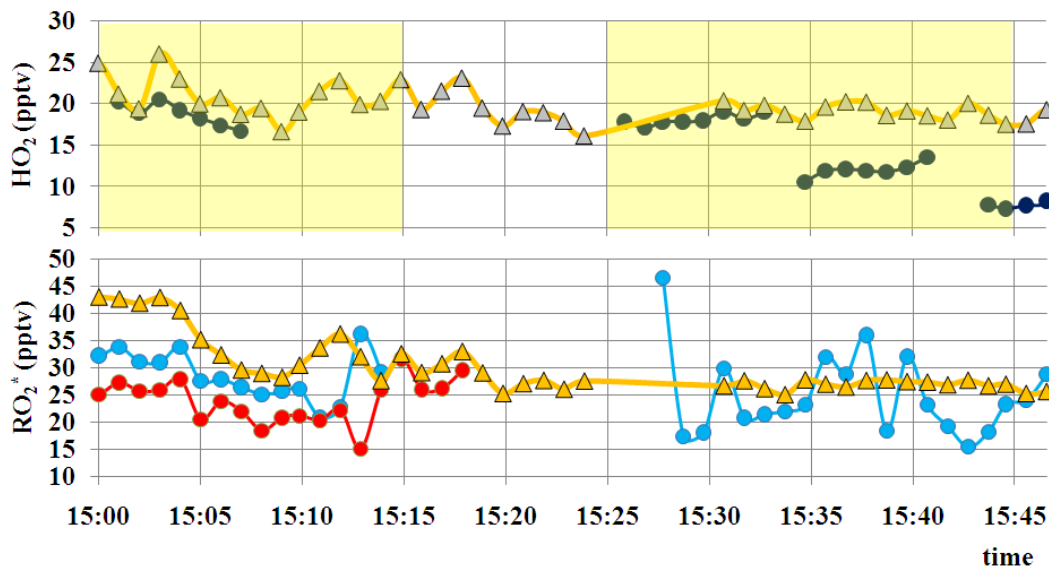
Fig. 7. Comparison of model and observations ( [\text{HO}_2] in dark blue, [\text{RO}_2^* -DUALER] in blue and [\text{RO}_2^* -PERCA 4] in red) for the 697 hPa pressure level during the intercomparison exercise. Model results (triangles) are constrained to j(\text{NO}_2) measured on board the D-Falcon scaled to the j(\text{NO}_2) -BAe values measured at 697 hPa. The periods of the intercomparison are highlighted in the top figure in yellow.
