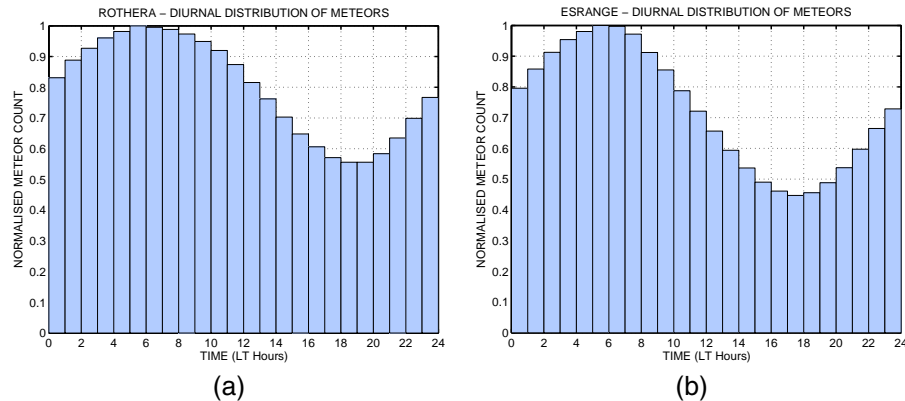
Fig. 2. Normalised diurnal variation in the meteor counts with respect to local time for the (a) Rothera meteor radar between 2005 and 2009 and (b) Esrang meteor radar between 1999 and 2009.
