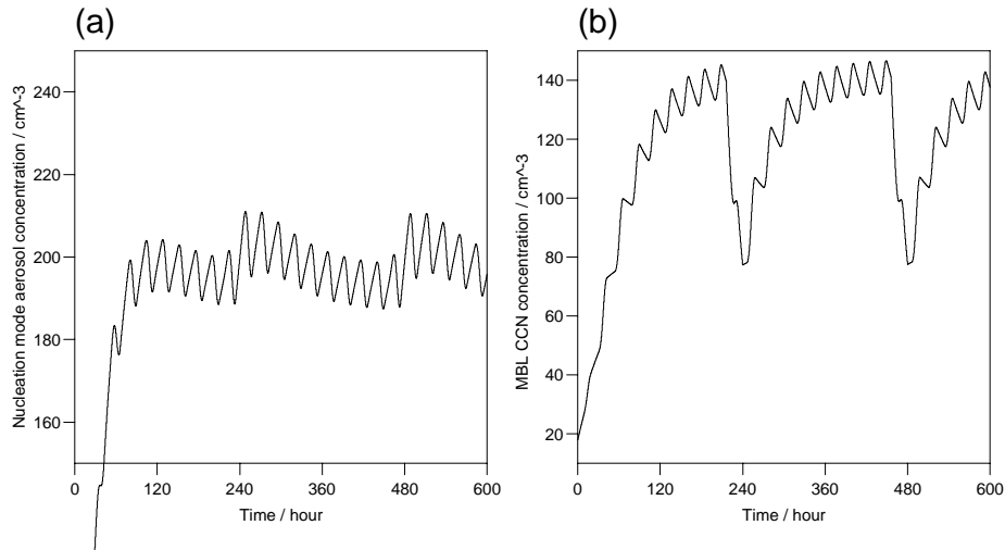
Fig. 4. Predicted variations in (a) nucleation and (b) accumulation mode aerosols. The entrainment terms were included in this case. The averaged concentration for N_1 and N_2 were 198 and 126 \text{ cm}^{-3} , respectively.
