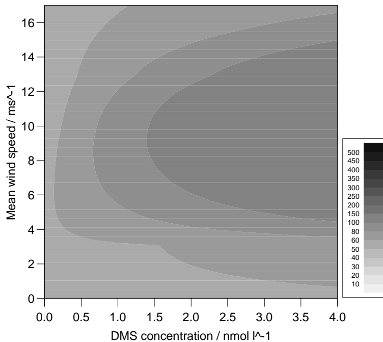
Fig. 8. Predicted CCN concentration (cm -3 ) when these are assumed to be composed of NSS CCN only. The flux of SS CCN was omitted in this simulation.
