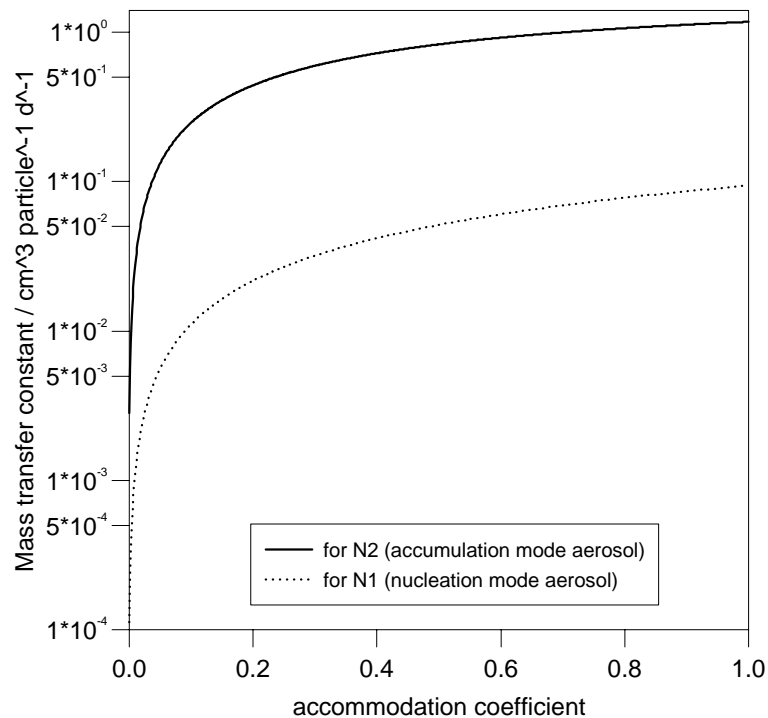
Fig. 3. Calculated mass transfer constant of sulfuric acids onto nucleation (dotted line) and accumulation mode (solid line) marine aerosols with various accommodation coefficients.
