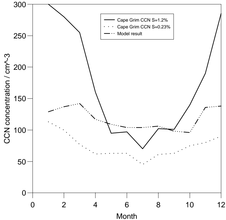
Fig. 9. Comparison of modelled results with Cape Grim CCN data. The dashed line is from the simulation. The solid and dotted line represent the CCN concentration for Cape Grim at 1.2 and 0.23% supersaturation, respectively.
